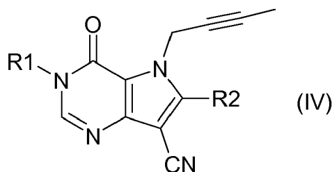
formula (IV)
