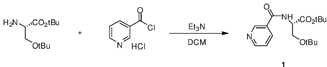
Scheme 1: Synthesis of nicotinoyl-Ser(tBu)OtBu 1
