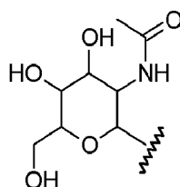
(N-acetyl-galactosamine)
