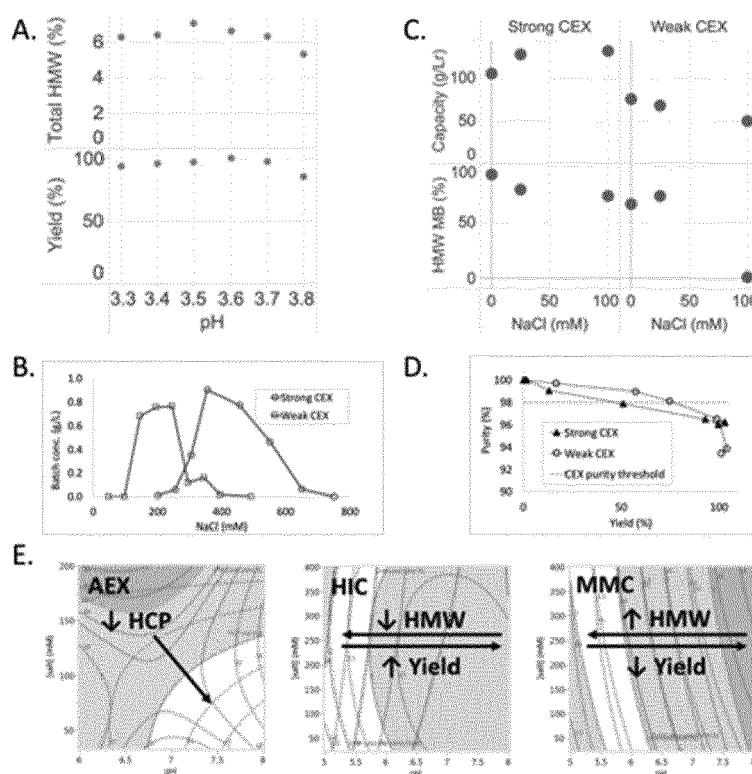
Figure 4. Example of data generated during a single batch binding experiment. Panel A: Protein A recovery vs. elution pH and pool HMW following a 60 minute low-pH hold. Panel B: Pseudo-chromatograms for 2 CEX resins. Panel C: Static capacity and HMW mass balance for 2 CEX resins. Panel D: Purity (HMW) plot for 2 CEX resins. Panel E: Recovery and contaminant contour plots for AEX, HIC, and MMC resins operated in flowthrough mode.
