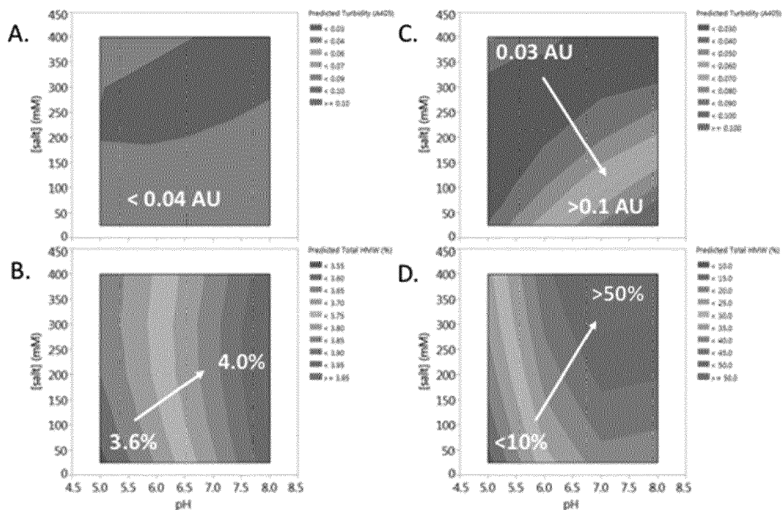
Figure 2. Comparison of solution stability for 2 mAbs for the range of downstream process conditions evaluated. Panels A and B present turbidity and HMW, respectively, for mAb 1. Panels C and D present turbidity and HMW for mAb 2.
