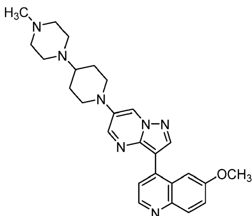
Compound 20
