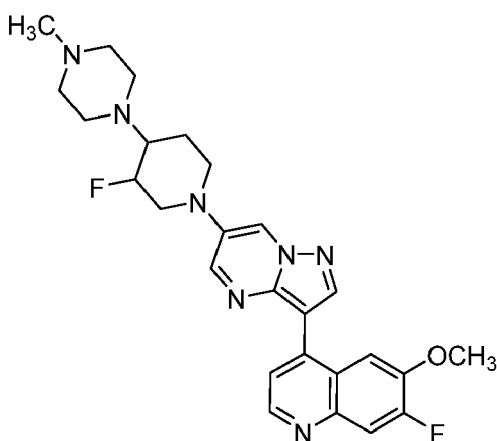
Compound 47
