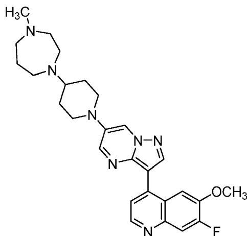
Compound 42
