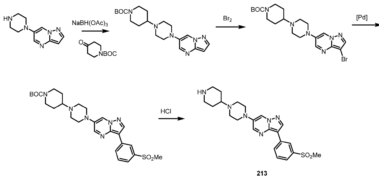
Compound 213
