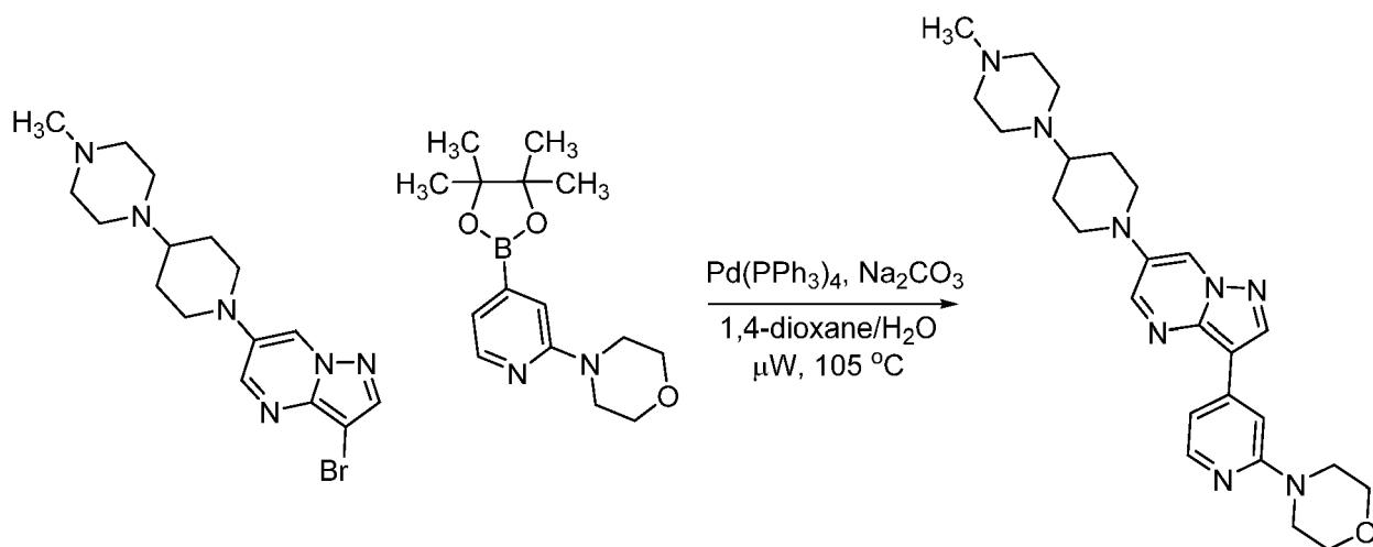
Compound 219
