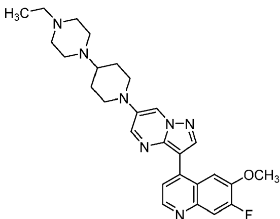
Compound 40
