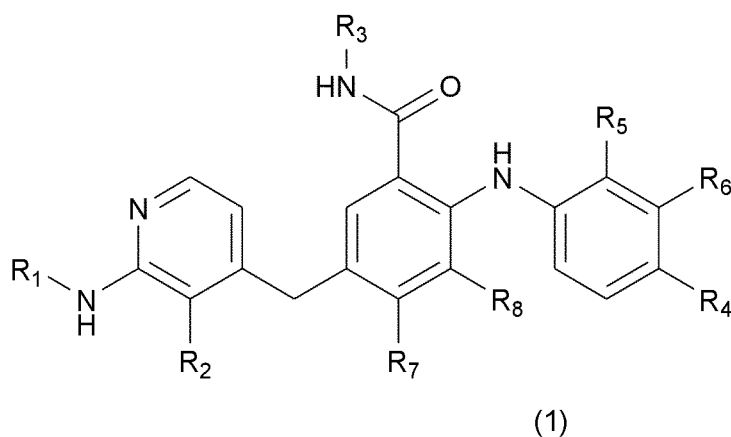
[Chemical Formula 7]
