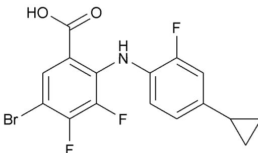
[Chemical Formula 25]
