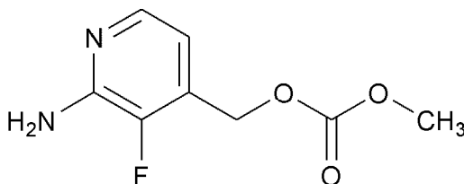
[Chemical Formula 23]
