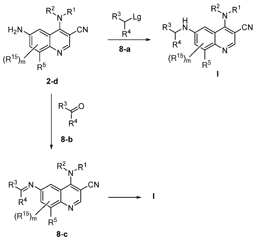
Scheme 8
