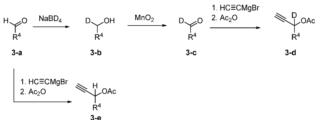
Scheme 3
