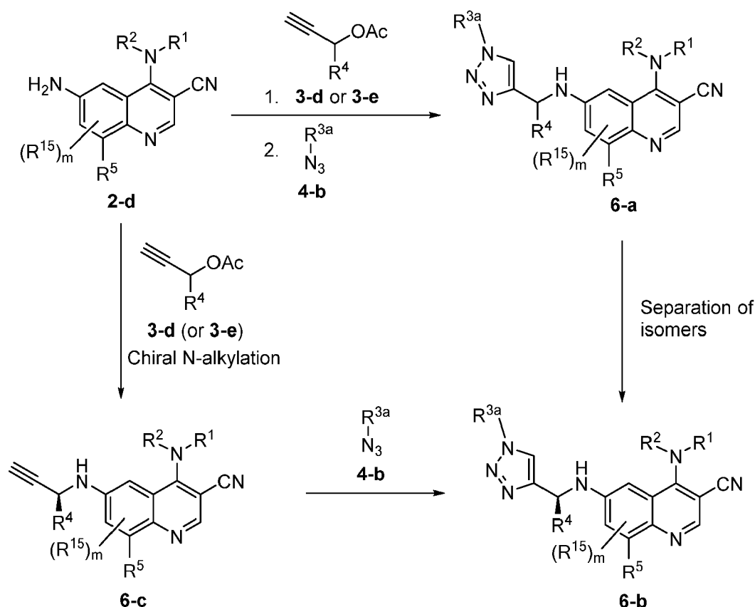
Scheme 6
