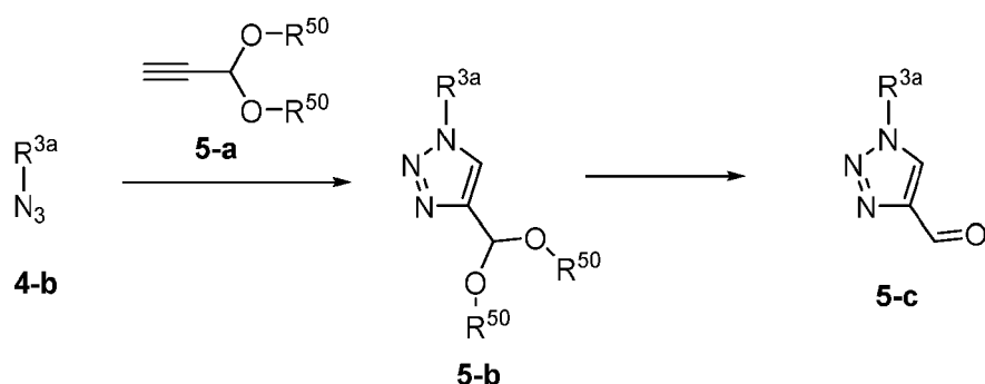
Scheme 5
