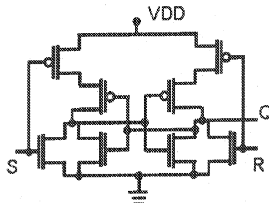
Compact CMOS Trigger Circuit
