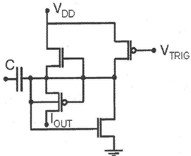
Compact CMOS Programmable Trigger Circuit
