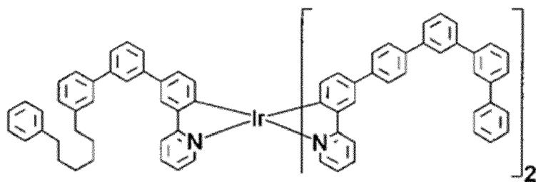
(Compound D-1)
