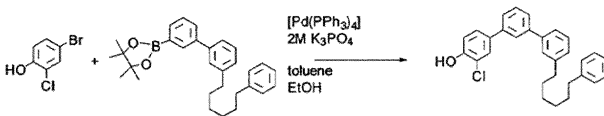
(Intermediate 3)
