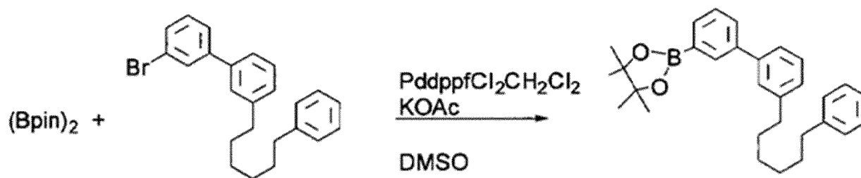
(Intermediate 1)
