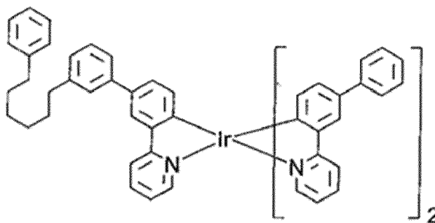
(Compound D-5)
