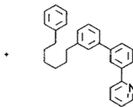
(Intermediate 14)
