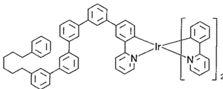
(Compound D-6)
