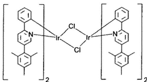
(Intermediate 13)
