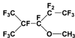
2-trifluoromethyl-3- methoxyperfluoropenta ne, (TMMP)
