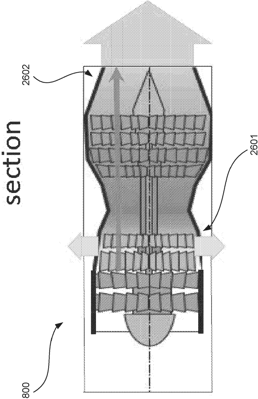
FIG. 26B :invented fluidic fan cross
