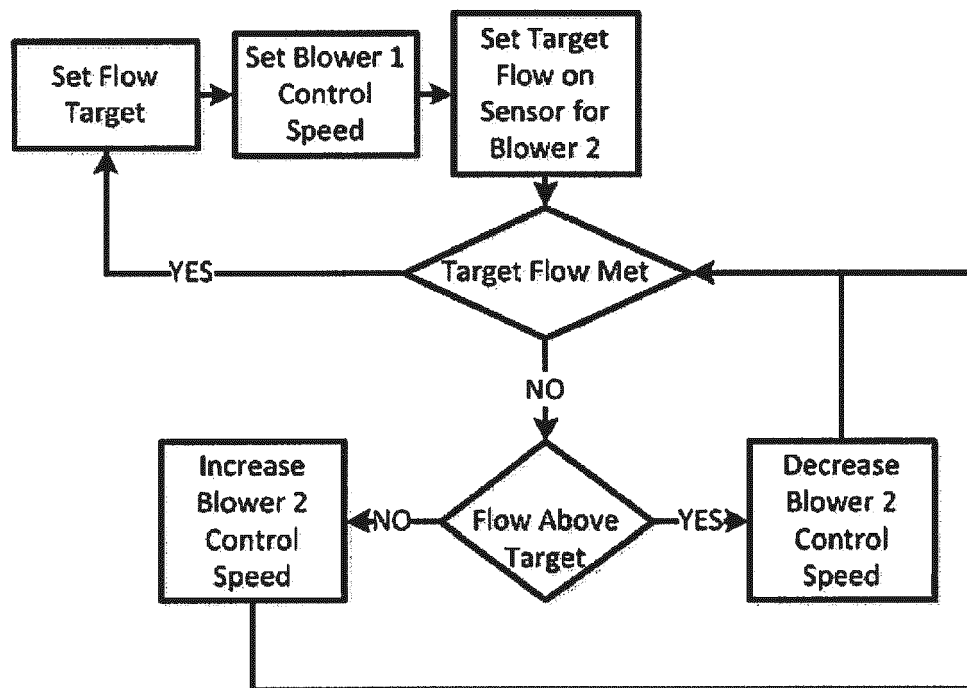
Fig. 11B Control Logic Diagram
