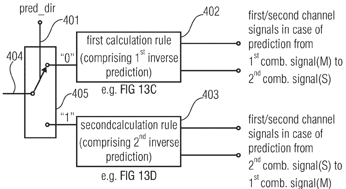
FIG 11B (DECODER SIDE)
