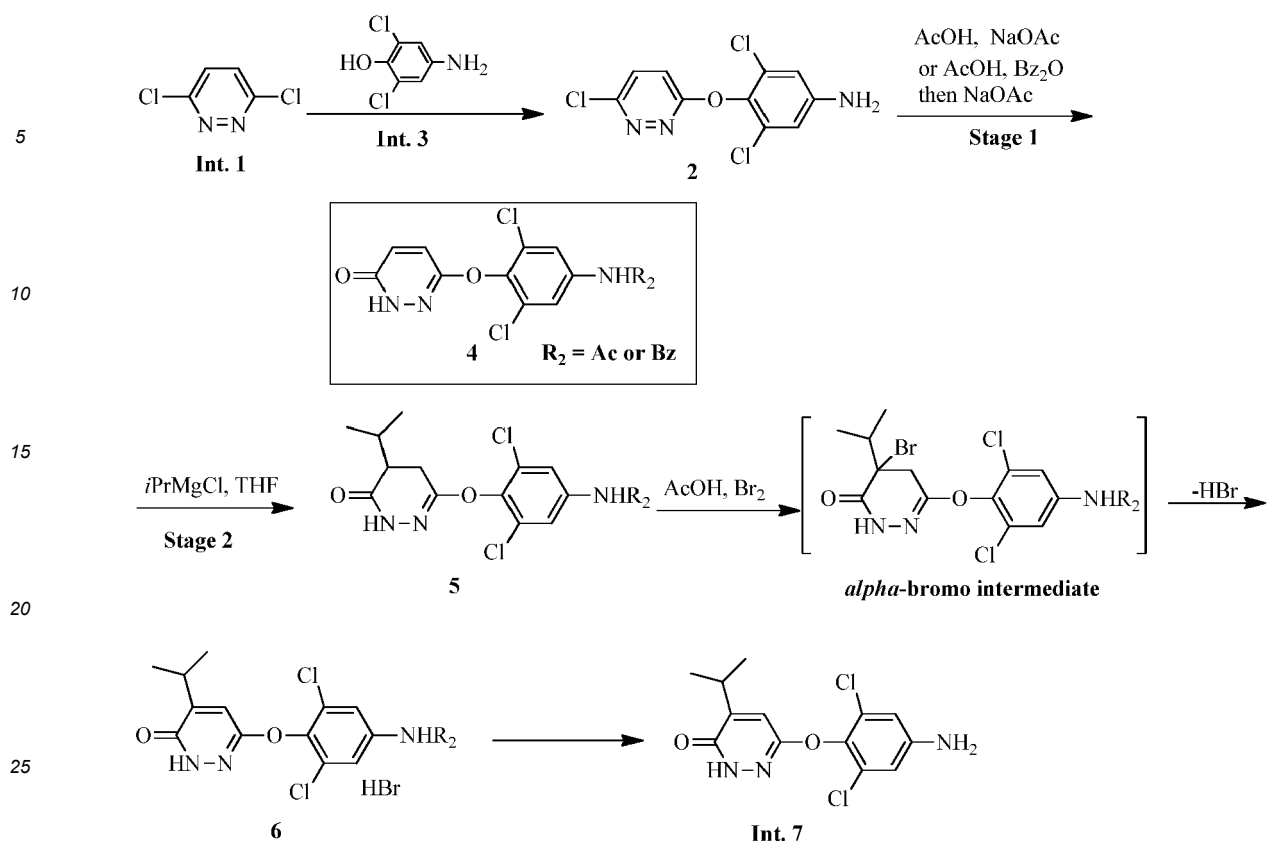
Scheme 2: Synthesis of 6-(4-amino-2,6-dichlorophenoxy)-4-isopropylpyridazin-3(2H)-one ( Int. 7 ) with isopropenyl Grignard reagent.
