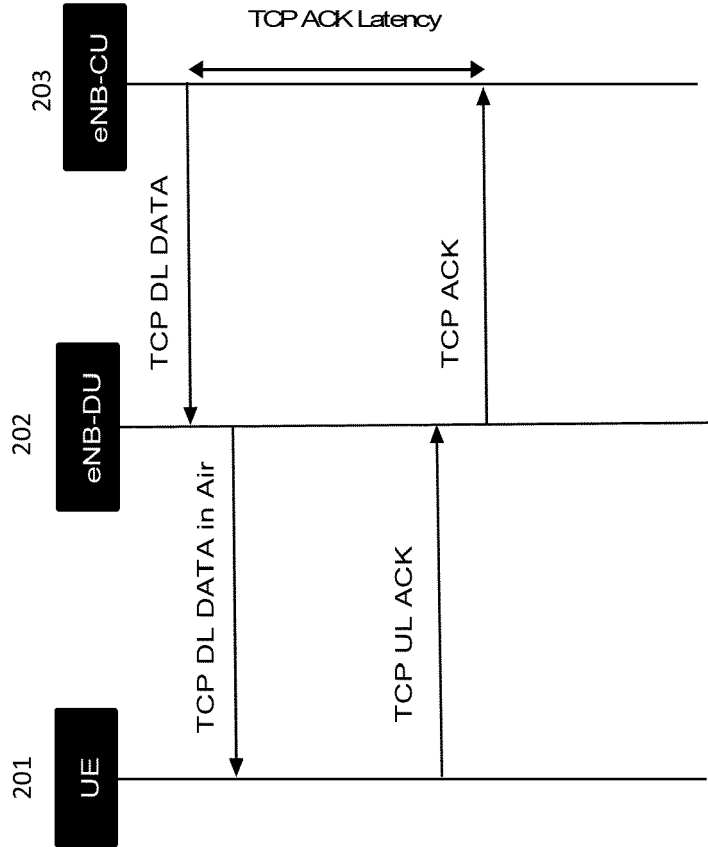
Diagram to illustrate the “TCP ACK latency”
