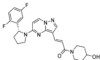
Chemical Compound 57
