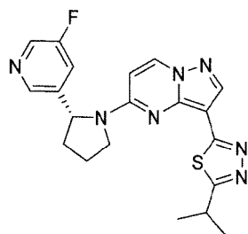
Chemical Compound 17
