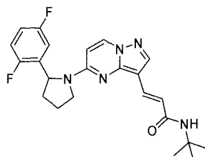
Chemical Compound 44
