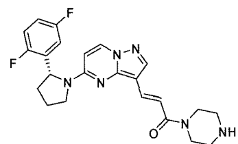
Chemical Compound 50
