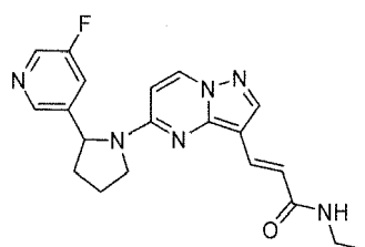
Chemical Compound 38
