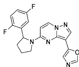
Chemical Compound 29
