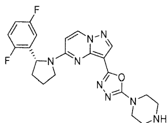
Chemical Compound 18
