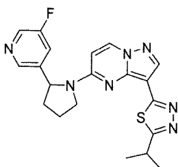
Chemical Compound 13
