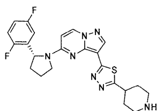
Chemical Compound 25
