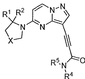
Formula IV
