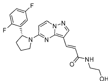
Chemical Compound 48
