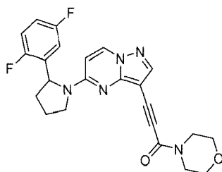
Chemical Compound 61.
