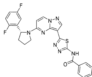
Chemical Compound 21
