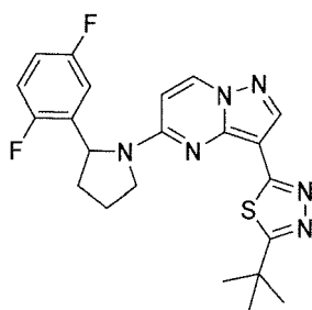
Chemical Compound 10
