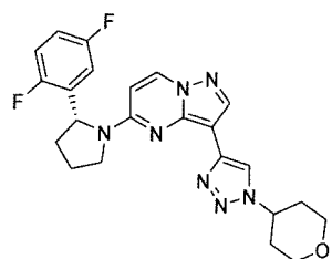
Chemical Compound 36
