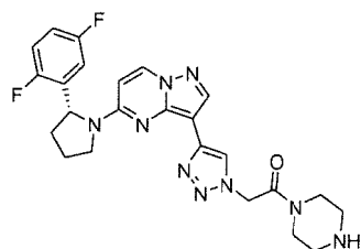
Chemical Compound 37
