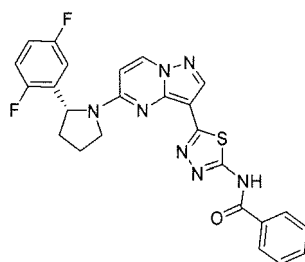
Chemical Compound 21
