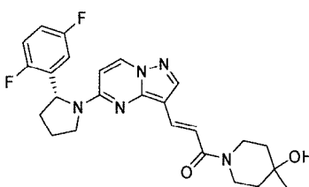
Chemical Compound 58
