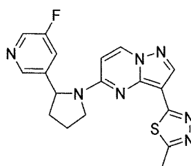
Chemical Compound 11
