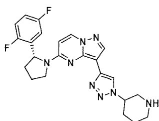
Chemical Compound 34
