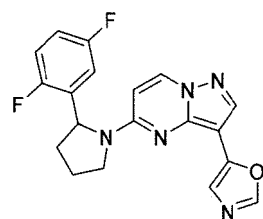
Chemical Compound 29
