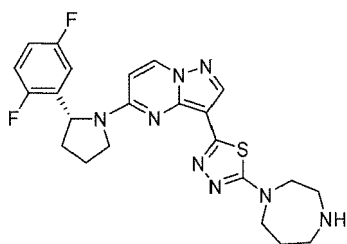
Chemical Compound 23
