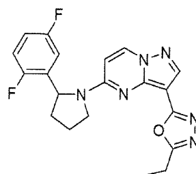
Chemical Compound 3
