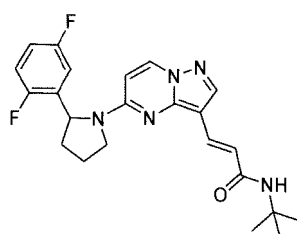
Chemical Compound 44
