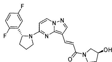
Chemical Compound 60
