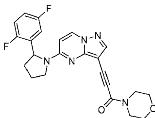
Chemical Compound 61
