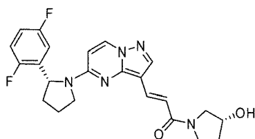
Chemical Compound 59
