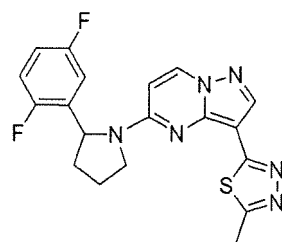
Chemical Compound 2
