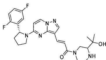
Chemical Compound 52
