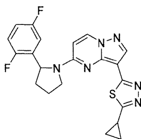
Chemical Compound 8
