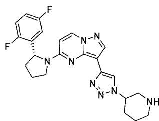
Chemical Compound 34
