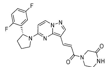
Chemical Compound 51
