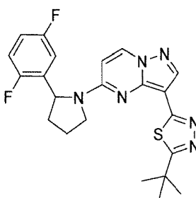
Chemical Compound 10
