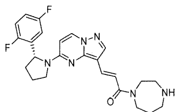
Chemical Compound 56
