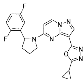
Chemical Compound 7
