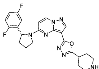
Chemical Compound 24
