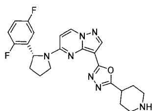
Chemical Compound 24
