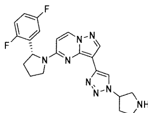
Chemical Compound 35
