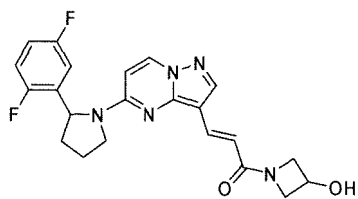
Chemical Compound 47
