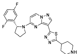
Chemical Compound 25
