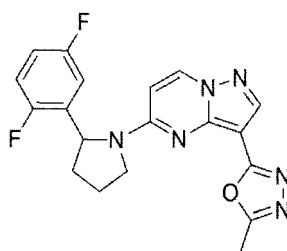
Chemical Compound 1
