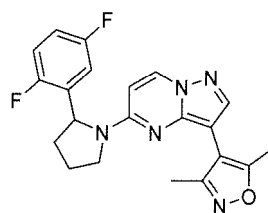
Chemical Compound 31
