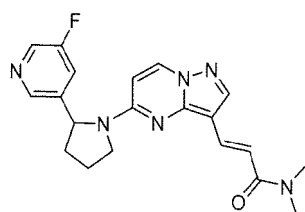
Chemical Compound 40
