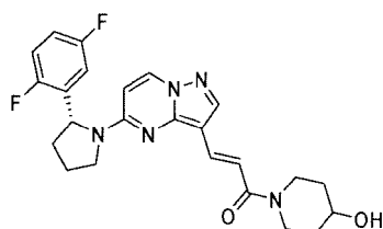
Chemical Compound 57
