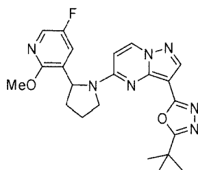
Chemical Compound 28
