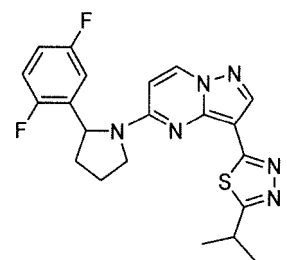
Chemical Compound 6
