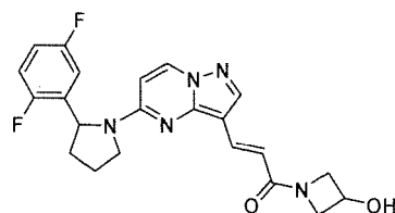
Chemical Compound 47
