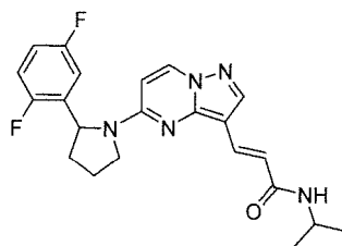
Chemical Compound 42
