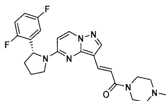
Chemical Compound 53
