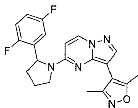
Chemical Compound 31
