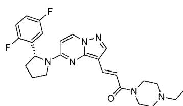
Chemical Compound 54
