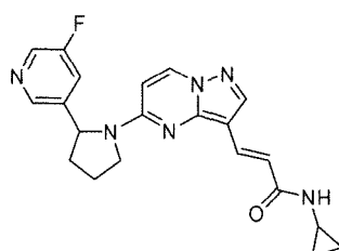
Chemical Compound 39
