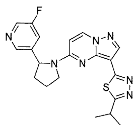
Chemical Compound 13
