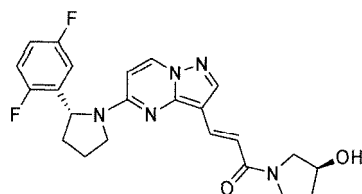
Chemical Compound 60
