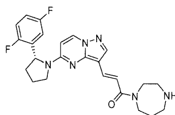
Chemical Compound 56
