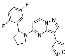
Chemical Compound 30
