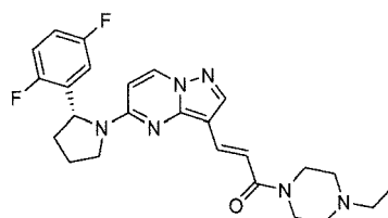
Chemical Compound 54
