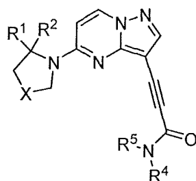
Formula IV
