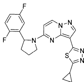
Chemical Compound 8
