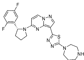
Chemical Compound 23
