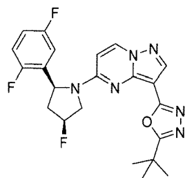
Chemical Compound 27
