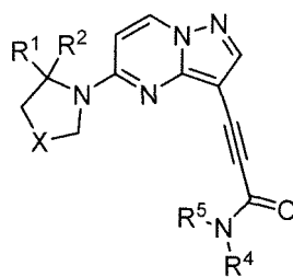
Formula IV.
