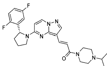
Chemical Compound 55
