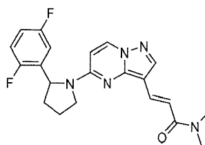
Chemical Compound 45
