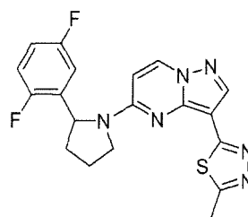
Chemical Compound 2
