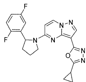
Chemical Compound 7
