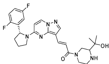
Chemical Compound 52
