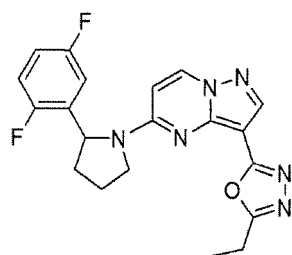
Chemical Compound 3
