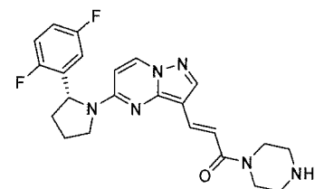
Chemical Compound 50
