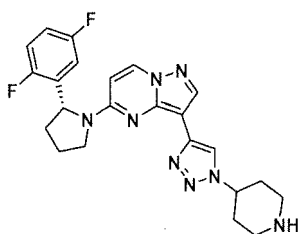
Chemical Compound 33
