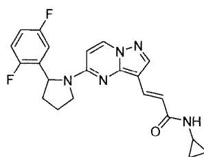
Chemical Compound 43
