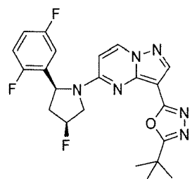
Chemical Compound 27
