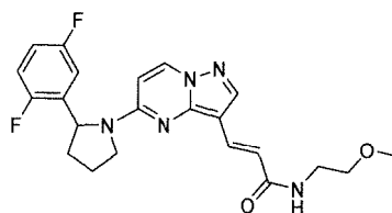
Chemical Compound 46
