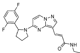
Chemical Compound 41
