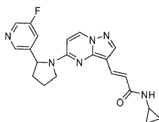
Chemical Compound 39
