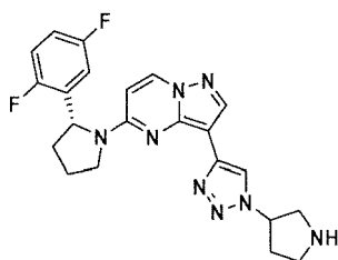
Chemical Compound 35
