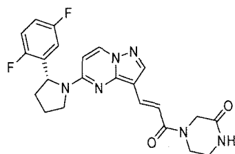
Chemical Compound 51
