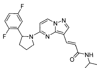
Chemical Compound 42
