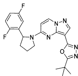
Chemical Compound 9
