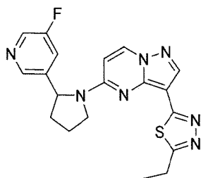
Chemical Compound 12
