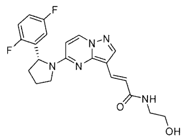
Chemical Compound 48
