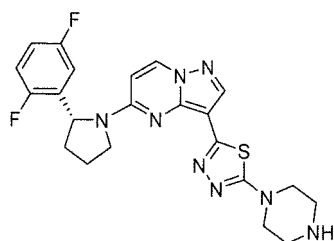
Chemical Compound 22
