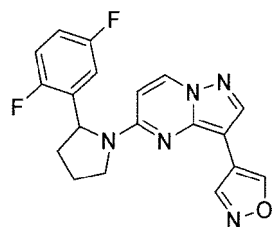
Chemical Compound 30
