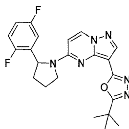
Chemical Compound 9
