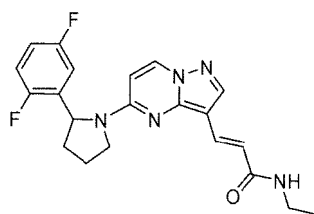
Chemical Compound 41
