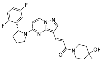
Chemical Compound 58
