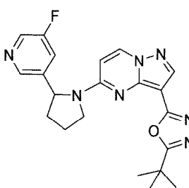
Chemical Compound 16
