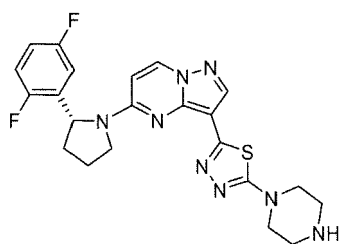
Chemical Compound 22
