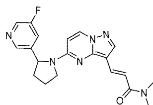
Chemical Compound 40
