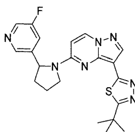
Chemical Compound 15
