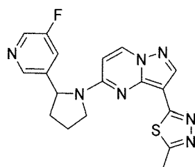
Chemical Compound 11
