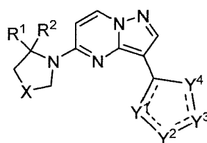
Formula III.
