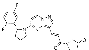
Chemical Compound 59
