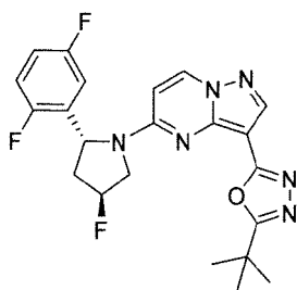
Chemical Compound 26
