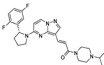
Chemical Compound 55
