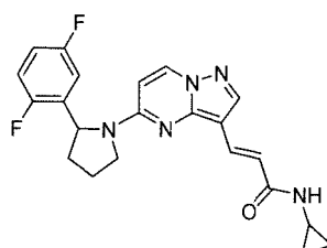
Chemical Compound 43
