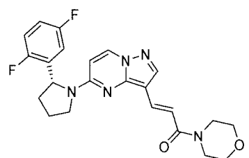
Chemical Compound 49
