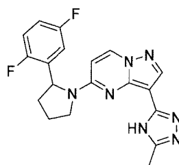
Chemical Compound 32
