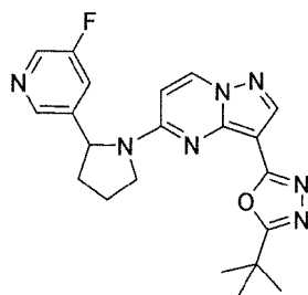
Chemical Compound 16
