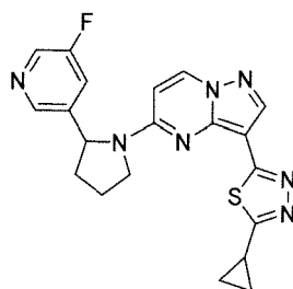
Chemical Compound 14
