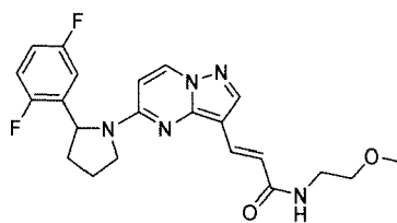
Chemical Compound 46
