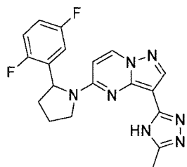
Chemical Compound 32
