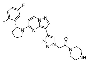
Chemical Compound 37
