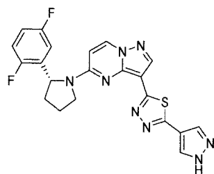
Chemical Compound 19
