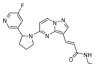
Chemical Compound 38
