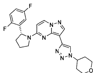
Chemical Compound 36
