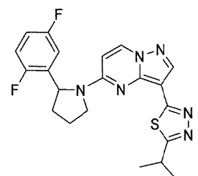
Chemical Compound 6
