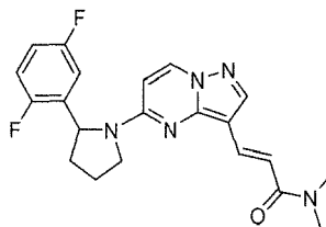
Chemical Compound 45
