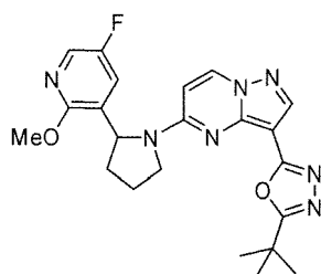
Chemical Compound 28
