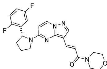
Chemical Compound 49
