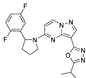
Chemical Compound 5
