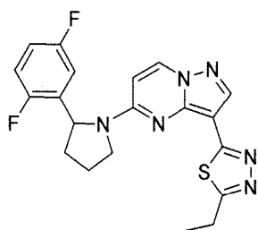
Chemical Compound 4
