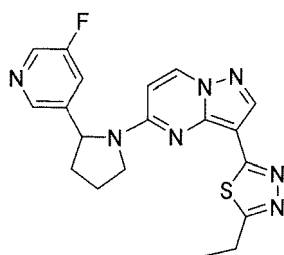
Chemical Compound 12
