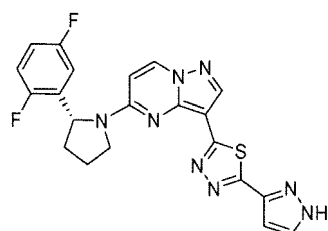
Chemical Compound 20
