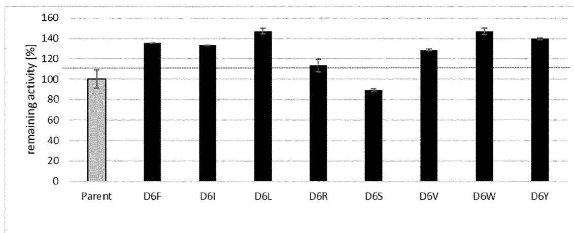
FIGURE 4. Remaining activity after NaOH incubation (pos. 6 modifications)
