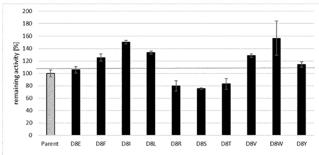
FIGURE 3. Remaining activity after NaOH incubation (pos. 4 modifications)
