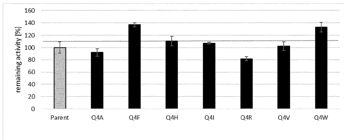
FIGURE 3. Remaining activity after NaOH incubation (pos. 4 modifications)
