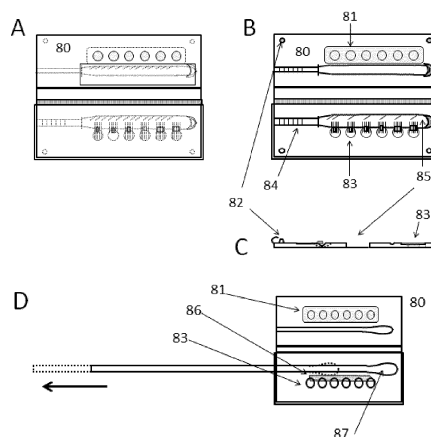
FIG. 33: Diagnostic swab device with housing
