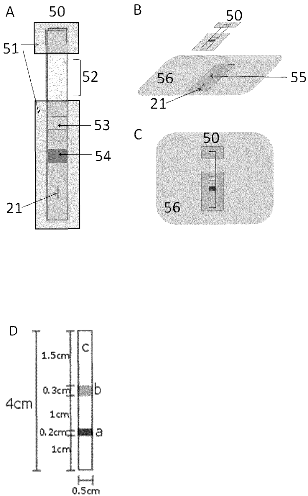
FIG. 15: Schematic of lysozyme test strip
