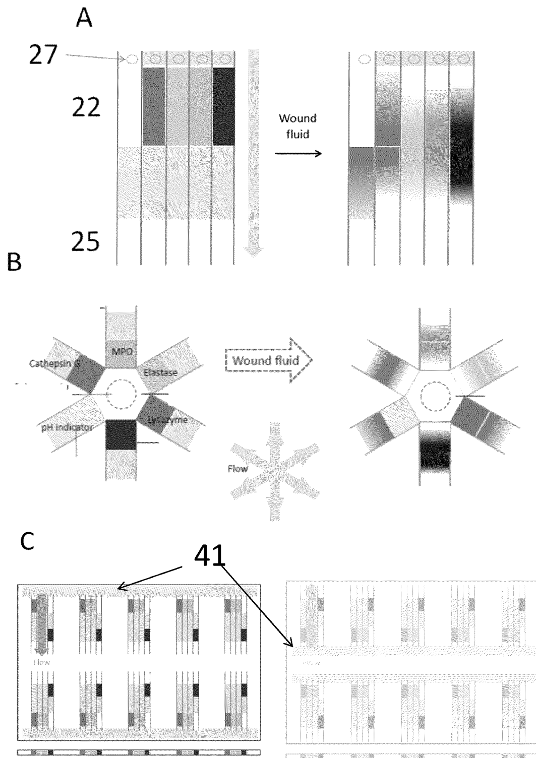
FIG. 4: Movement of indicators in reaction cells
