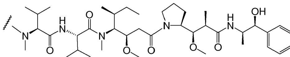
MMAE
