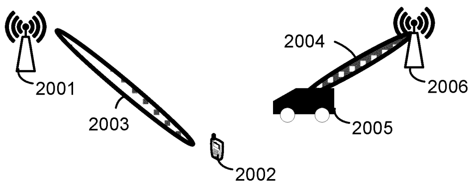
FIG. 20B Beam failure in multiple TRPs
