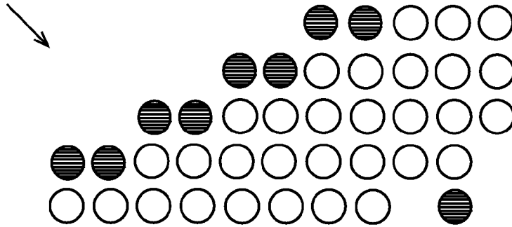
Truncated Radix-4 Booth Array 3104
