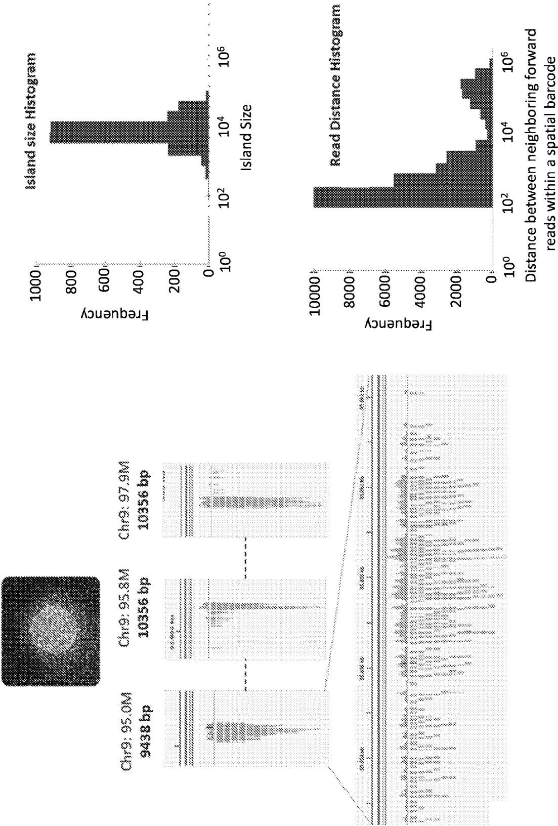
FIG. 8 Sequence reads from a single bead
