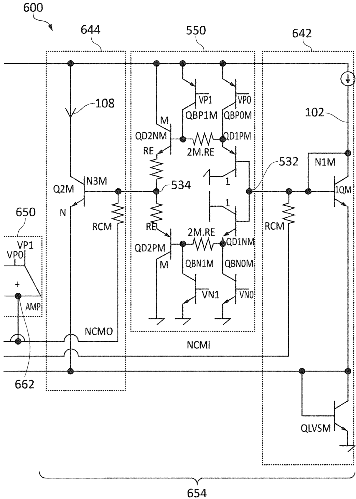
FIG. 6 (continued)
