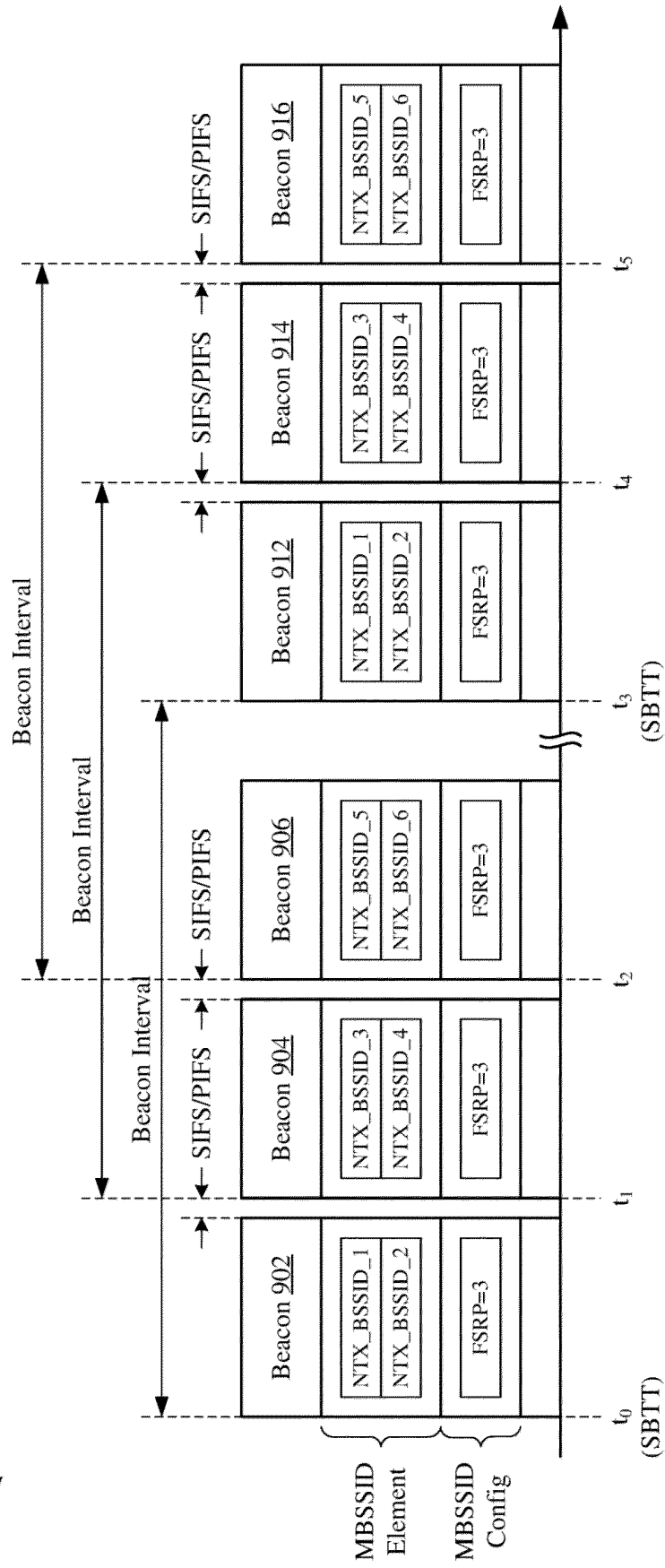
Figure 9
