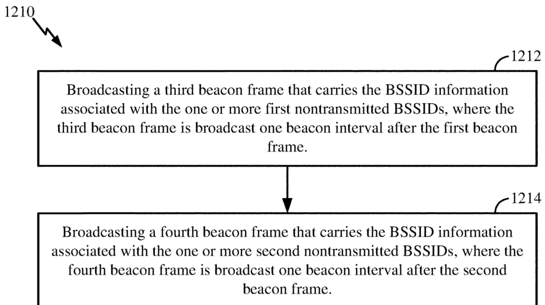
Figure 12B
