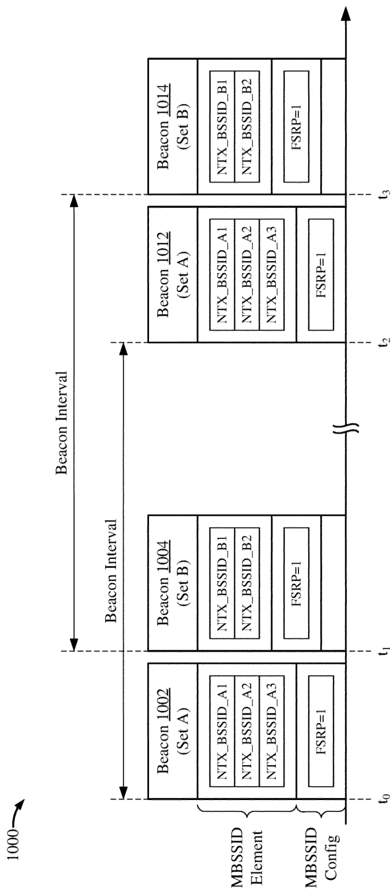
Figure 10
