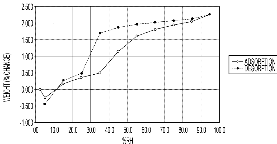
FIG. 24. DVS of Compound I Fumaric Acid
