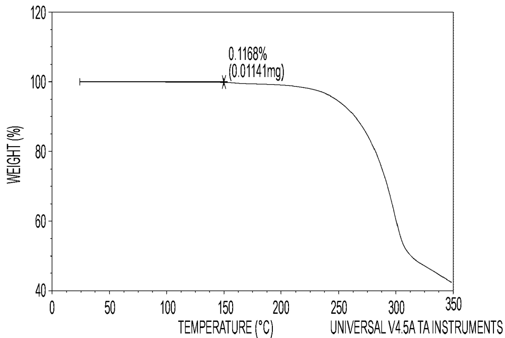
FIG. 3. TGA curve for Compound I Form I
