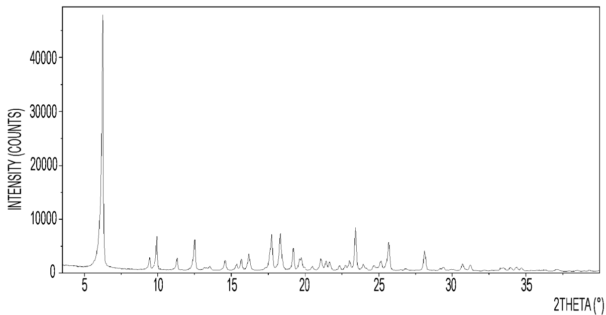
FIG. 13. XRPD pattern of Compound I Tartaric Acid
