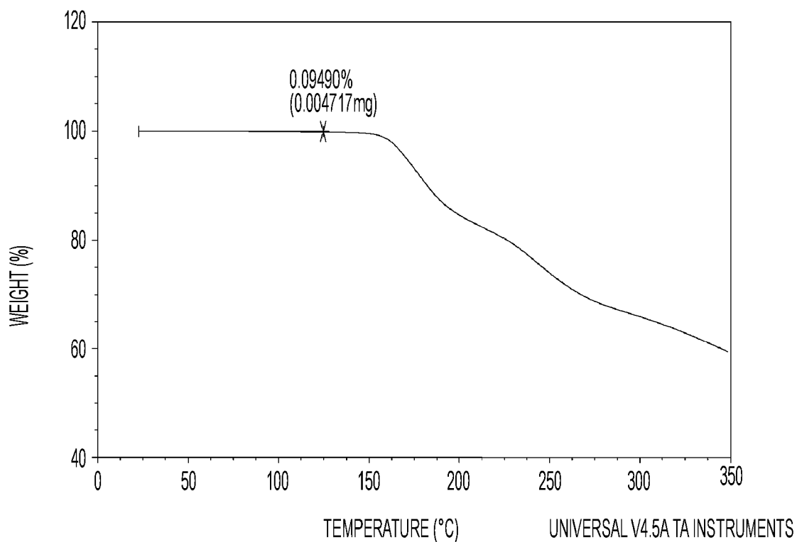
FIG. 19. TGA of Compound I Maleic Acid
