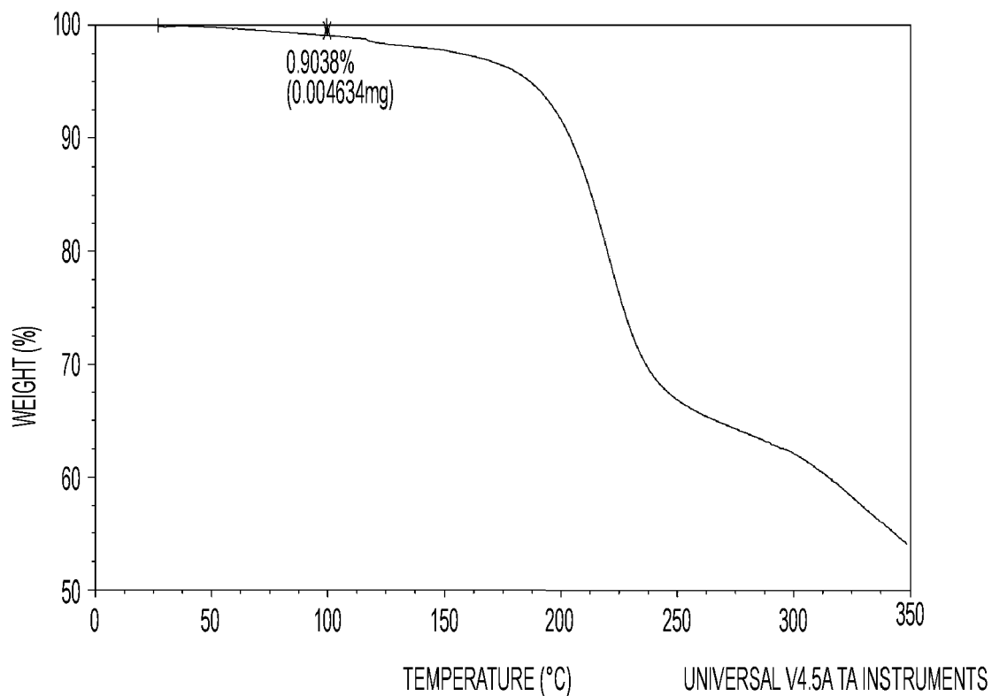
FIG. 15. TGA of Compound I Tartaric Acid
