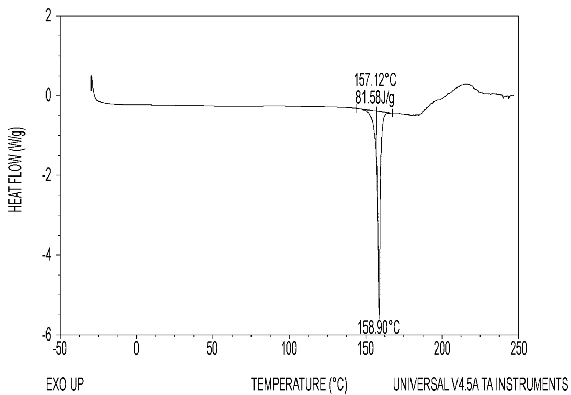
FIG. 14. DSC of Compound I Tartaric Acid
