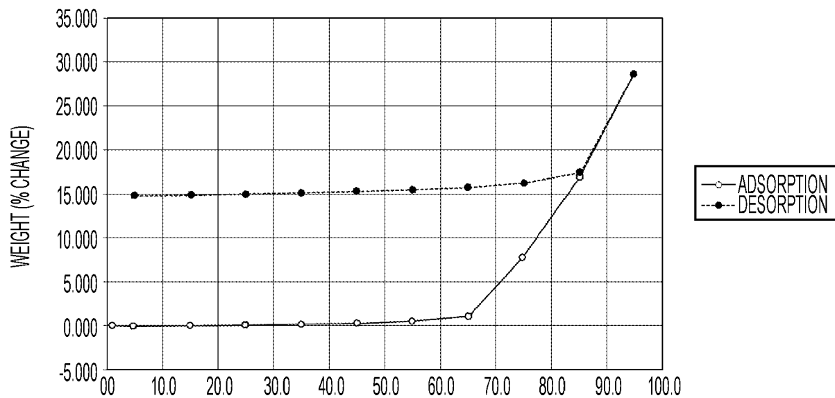
FIG. 8. DVS of Compound I HCl Form I
