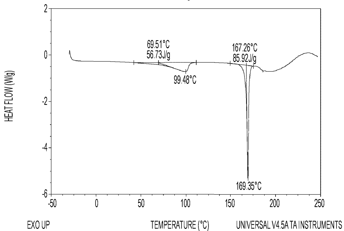
FIG. 22. DSC of Compound I Fumaric Acid
