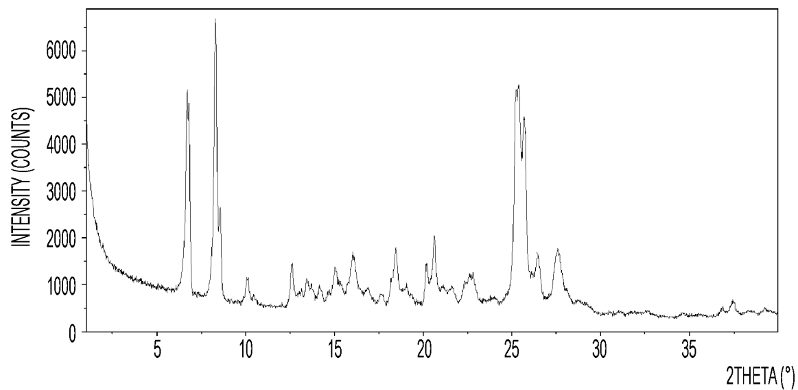
FIG. 21. XRPD pattern of Compound I Fumaric Acid
