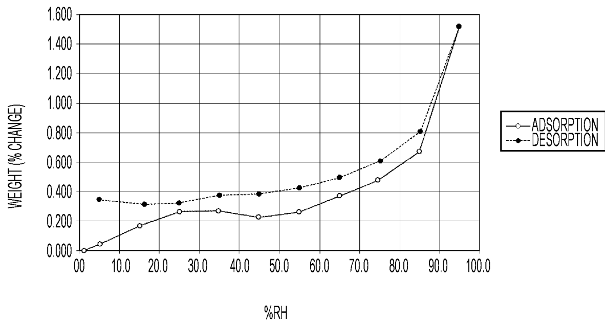
FIG. 16. DVS of Compound I Tartaric Acid
