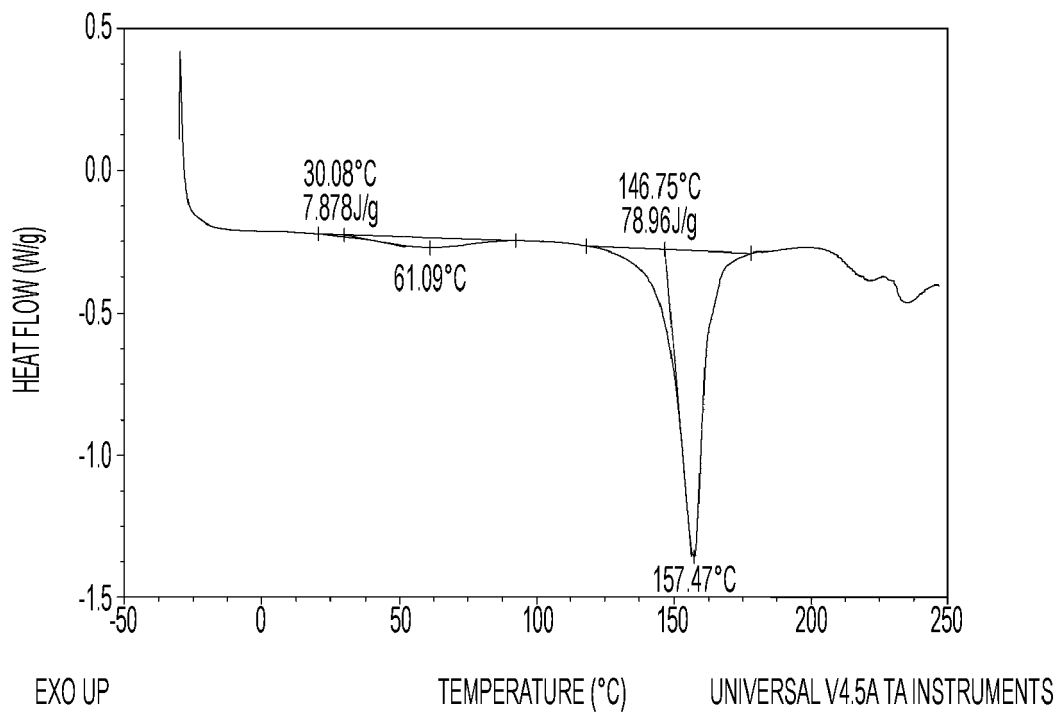
FIG. 26. DSC of Compound I Methanesulfonic Acid
