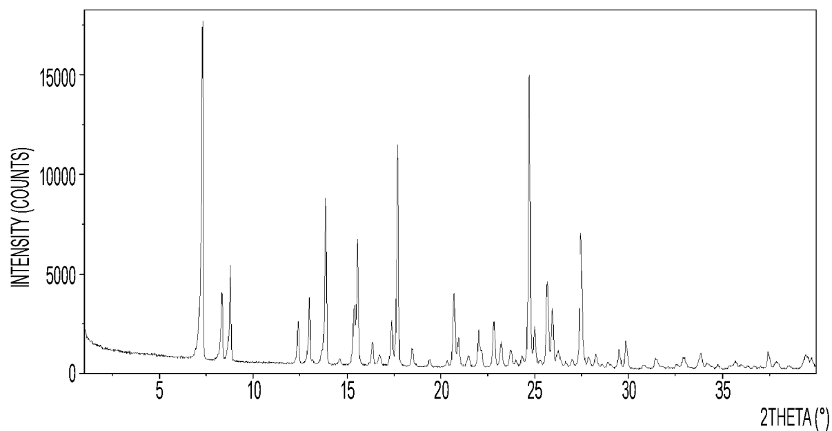
FIG. 17. XRPD pattern of Compound I Maleic Acid
