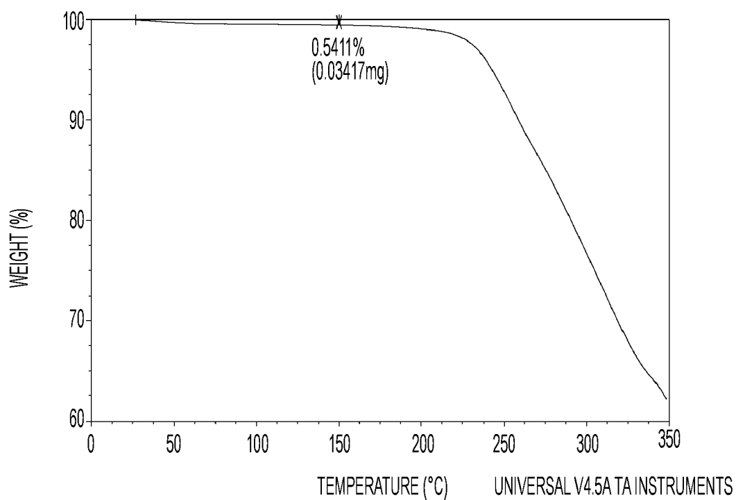
FIG. 27. TGA of Compound I Methanesulfonic Acid
