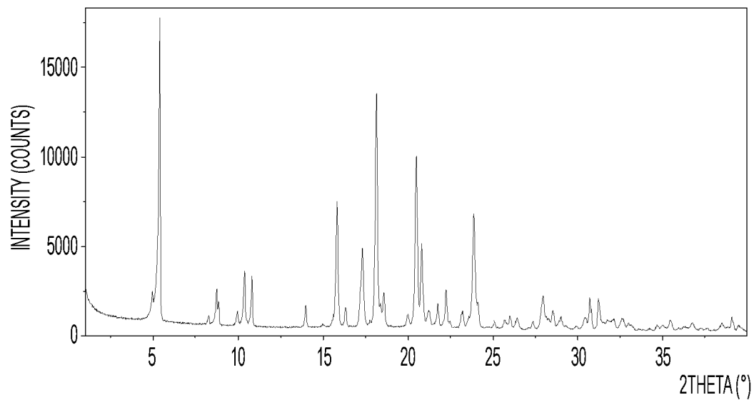
FIG. 25. XRPD pattern of Compound I Methanesulfonic Acid
