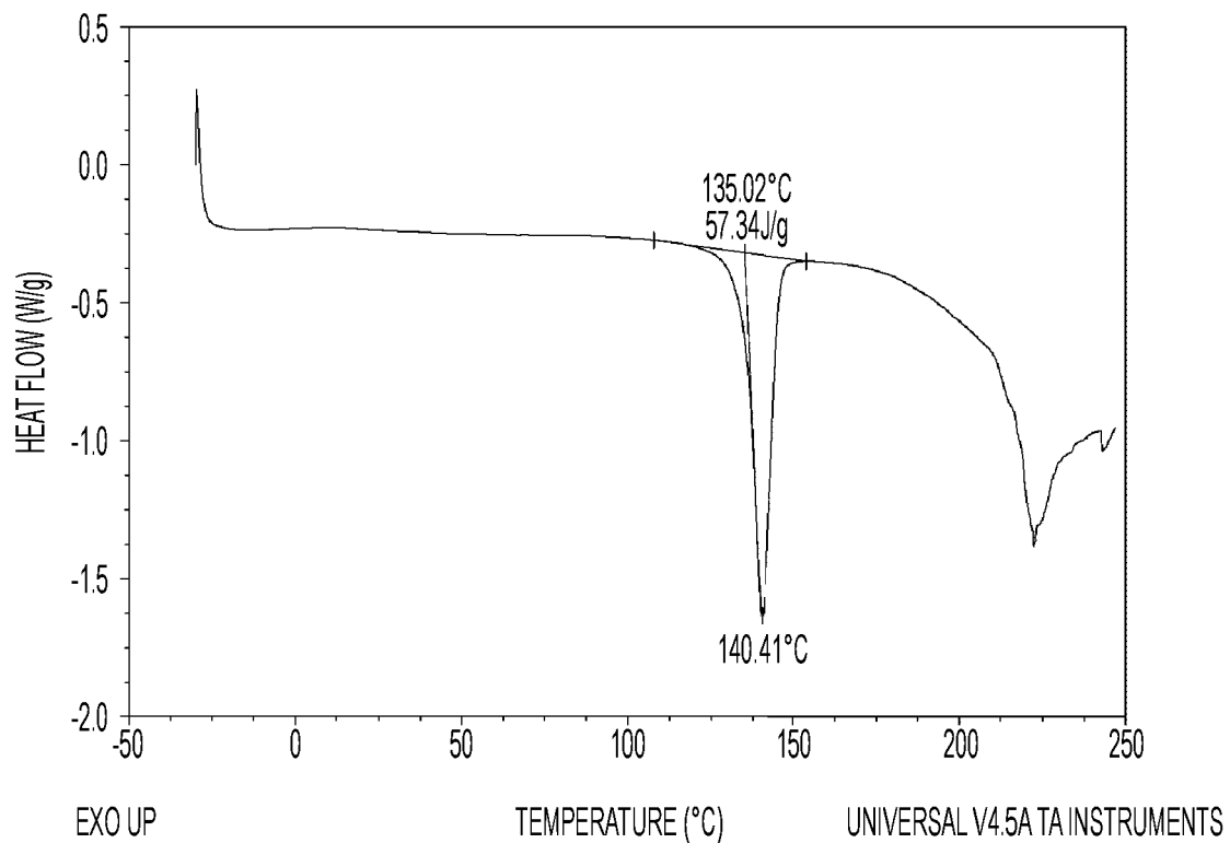
FIG. 6. DSC of Compound I HCl Form I
