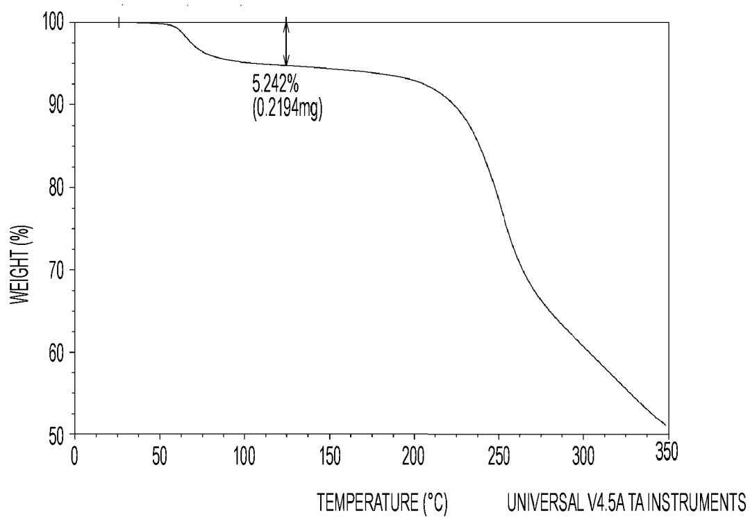
FIG. 11. TGA of Compound I HCl Form II
