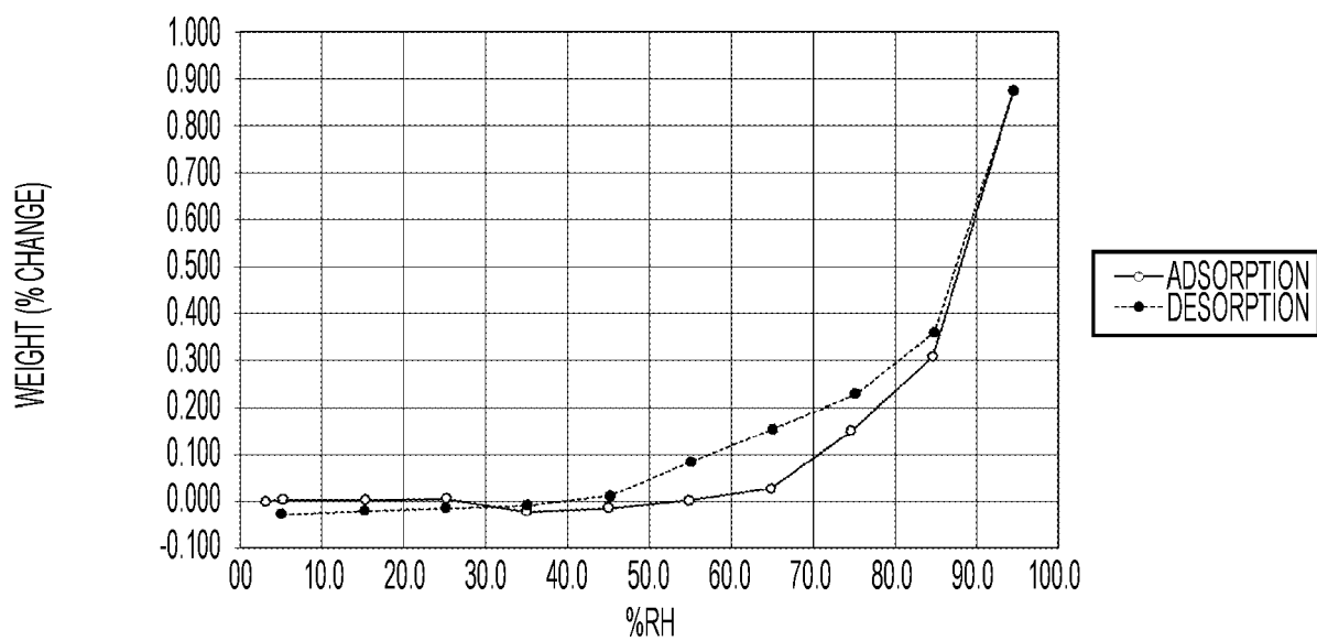
FIG. 4. DVS curve for Compound I Form I
