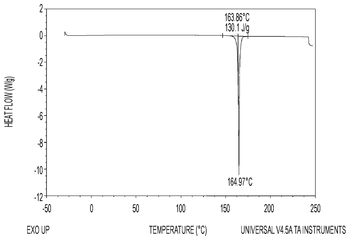
FIG. 2. DSC of Compound I Form I
