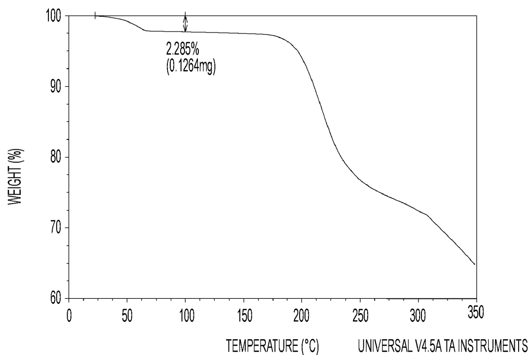
FIG. 23. TGA of Compound I Fumaric Acid
