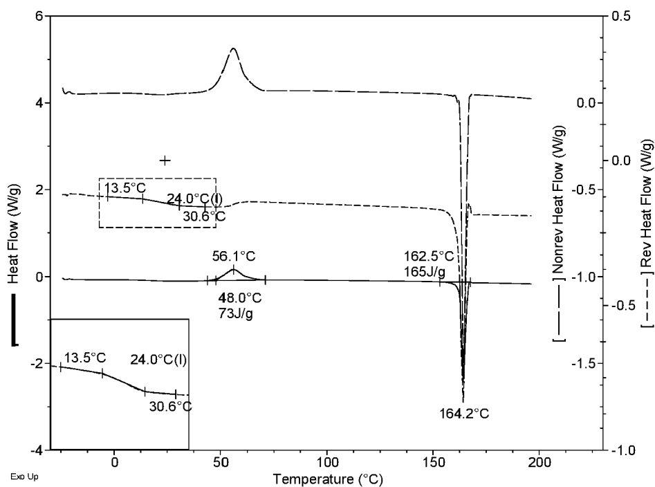
FIG. 30. DSC curve for Compound I Amorphous
