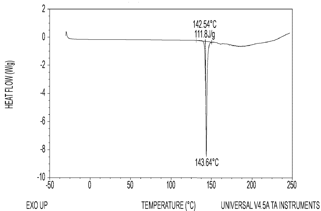
FIG. 18. DSC of Compound I Maleic Acid
