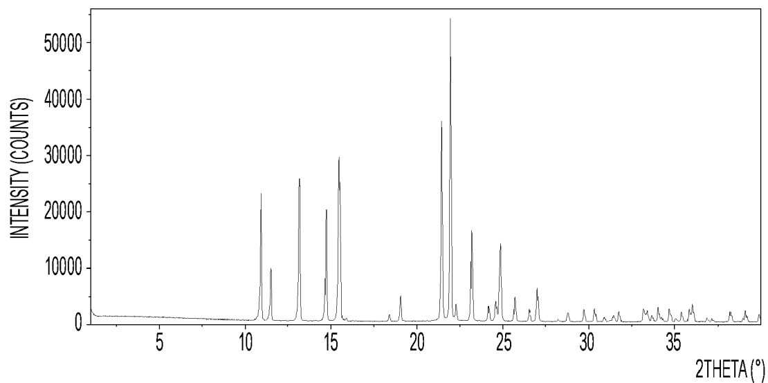
FIG. 1. XRPD pattern of Compound I Form I
