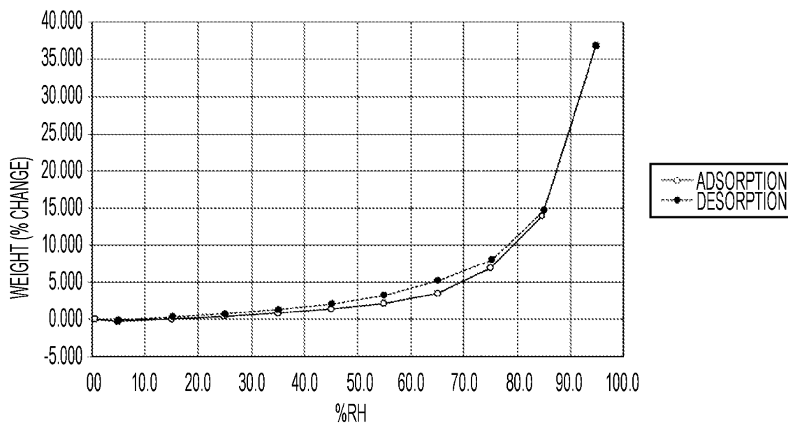
FIG. 28. DVS of Compound I Methanesulfonic Acid
