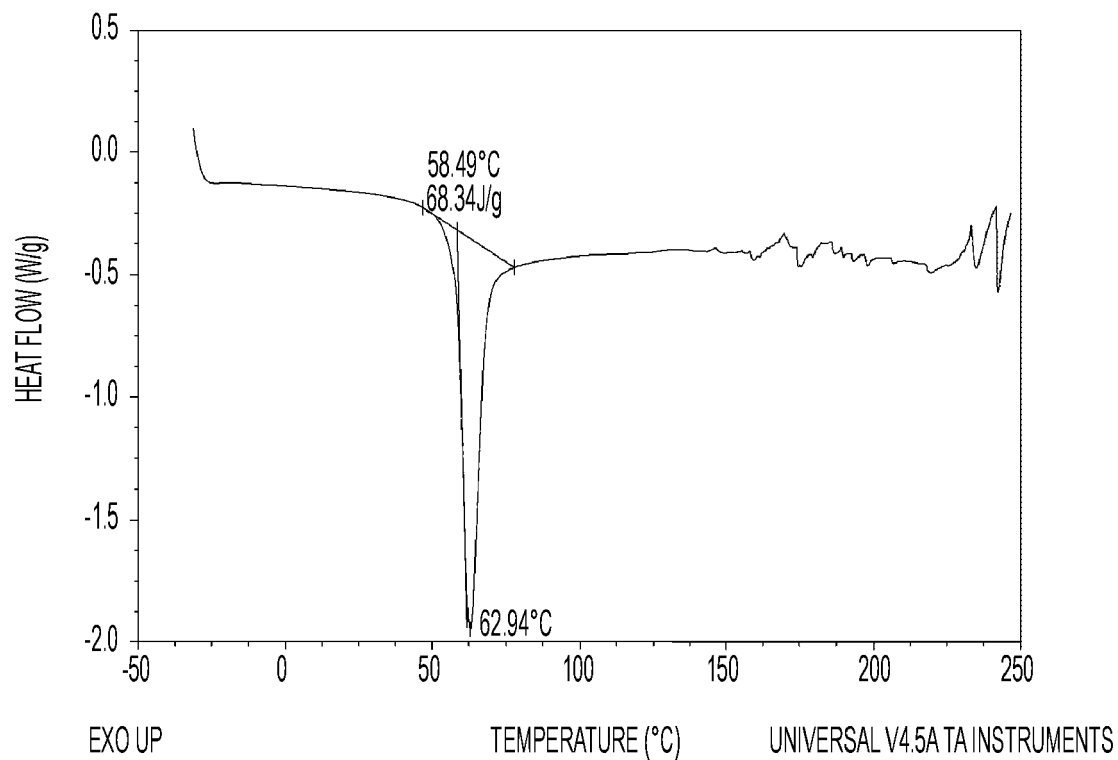
FIG. 10. DSC of Compound I HCl Form II
