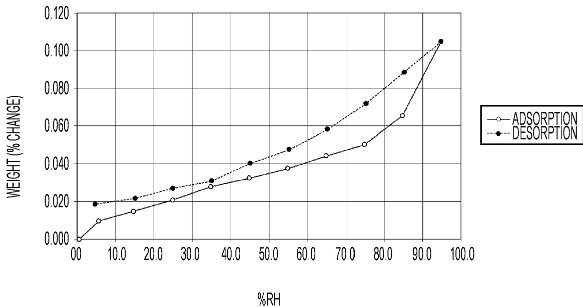
FIG. 20. DVS of Compound I Maleic Acid
