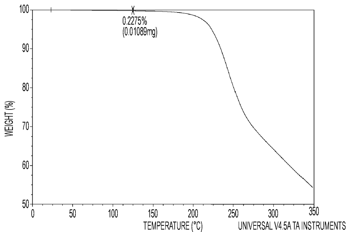
FIG. 7. TGA of Compound I HCl Form I
