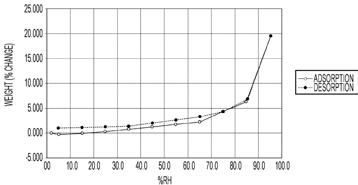
FIG. 12. DVS of Compound I HCl Form II
