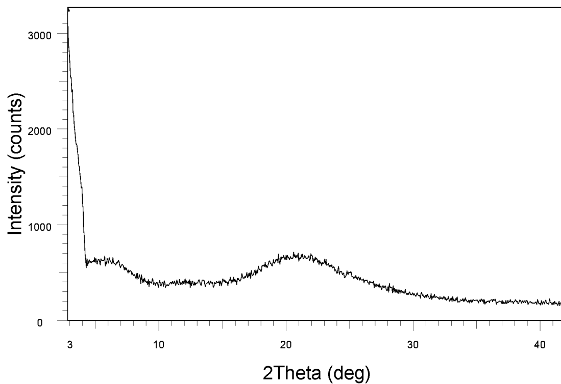
FIG. 29. XRPD pattern for Compound I Amorphous
