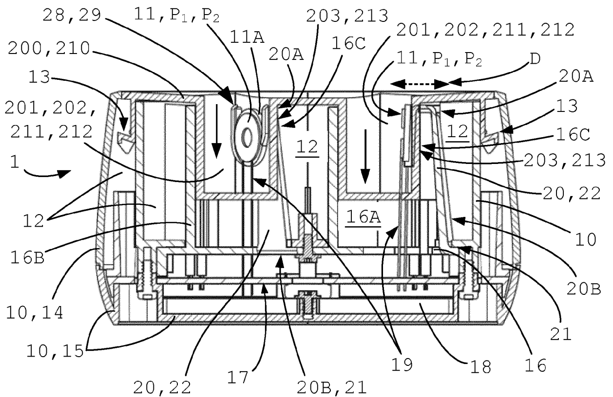
Fig 8B (B-B)
