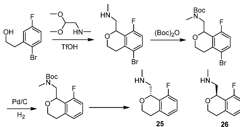
(a). 1-(5-bromo-8-fluoroisochroman-1-yl)-N-methylmethanamine
