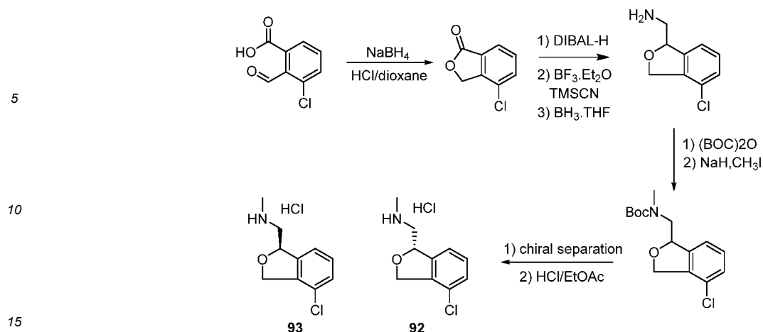
(a). 4-chloroisobenzofuran-1(3H)-one
