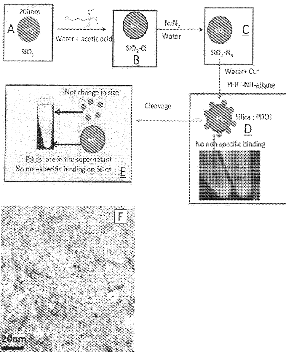
TEM image of the Pdots obtained from Step E
