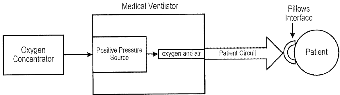
FIG. 1 (PRIOR ART)
