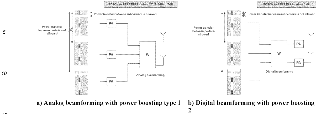
Figure 3. Example of power boosting type 1 and 2 for a transmission with 2 PTRS ports, 3 DMRS ports and 3 PDSCH layers.
