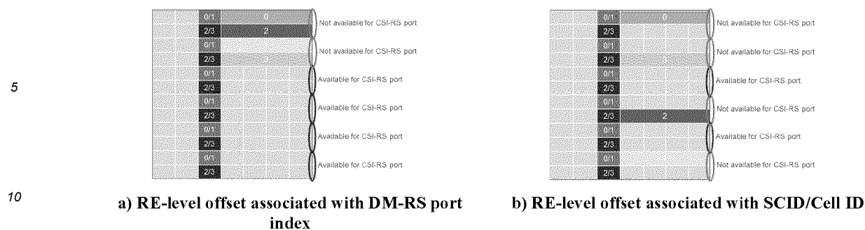
Figure 1. Example of PTRS fixed and configurable mapping and the available CSI-RS ports.
