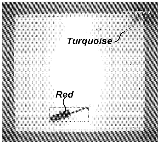
Visible Light
