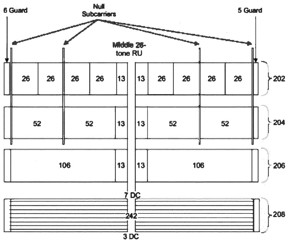
FIGURE 2A (Prior Art)
