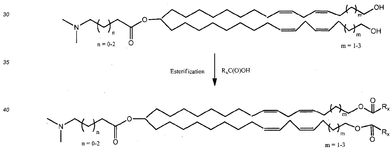
Scheme G
