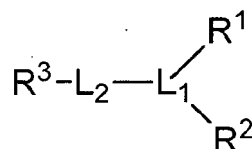
Formula (IE)
