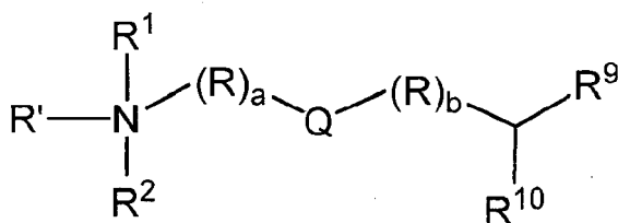
Formula (IC)
