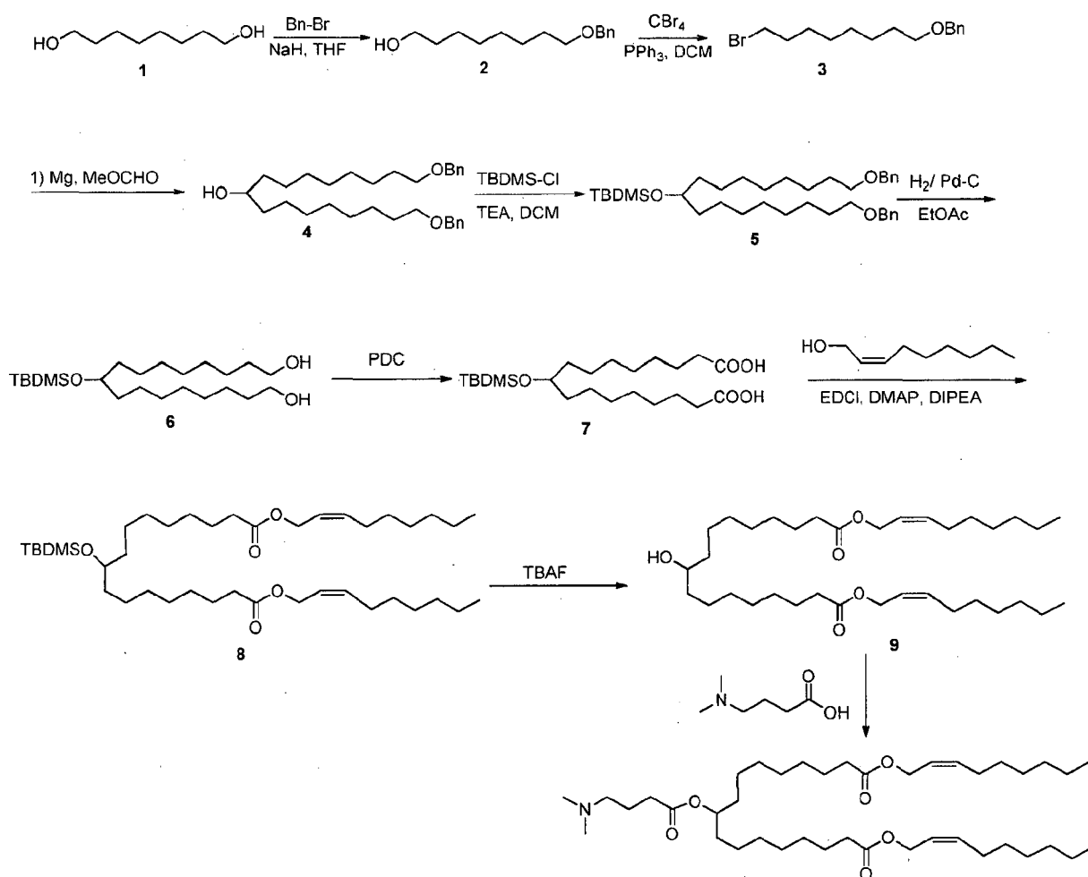
Scheme 7:
