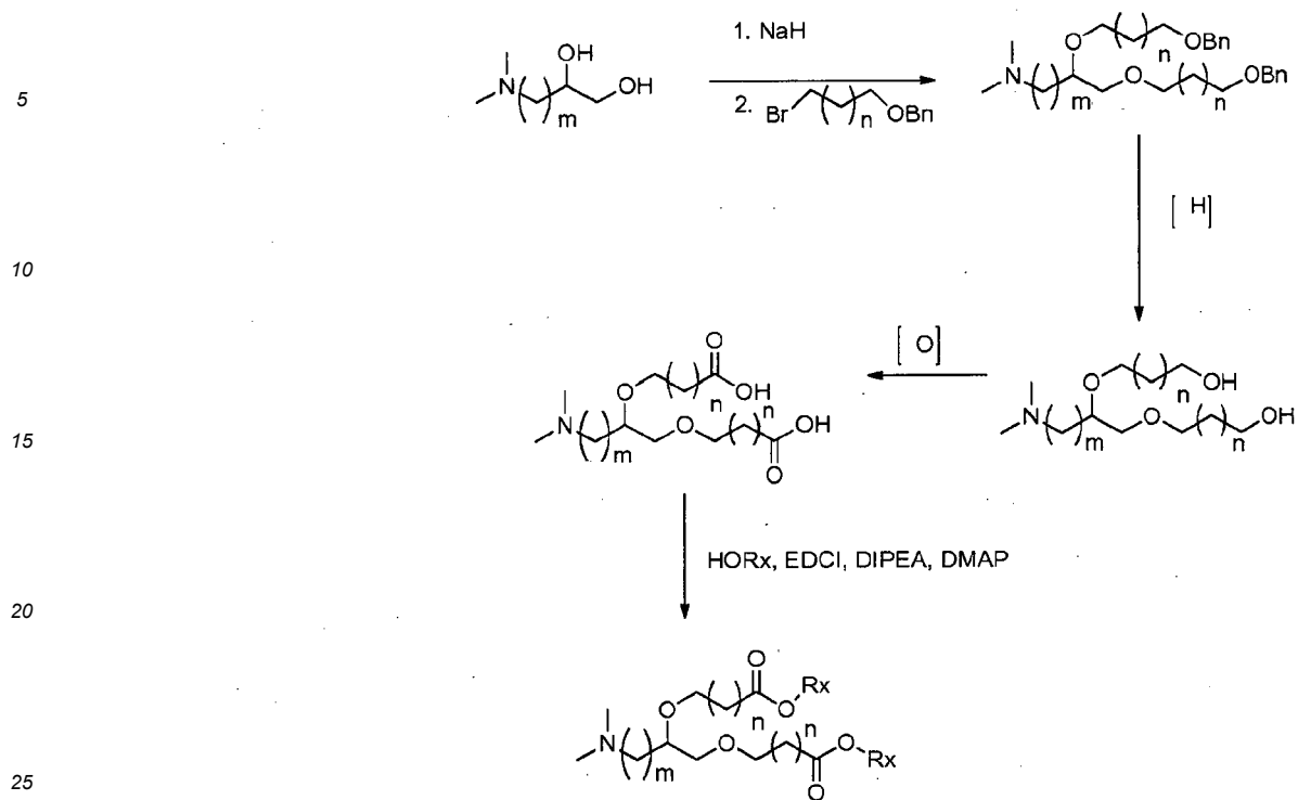
Scheme F
