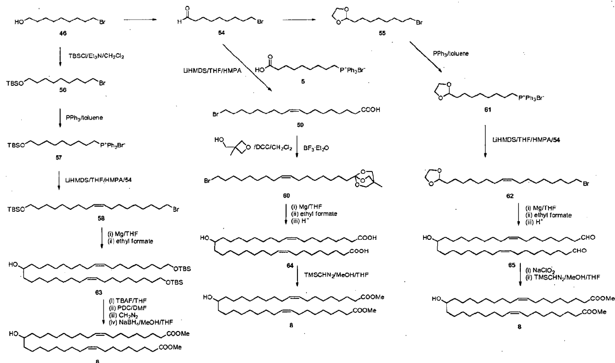
Scheme 6
