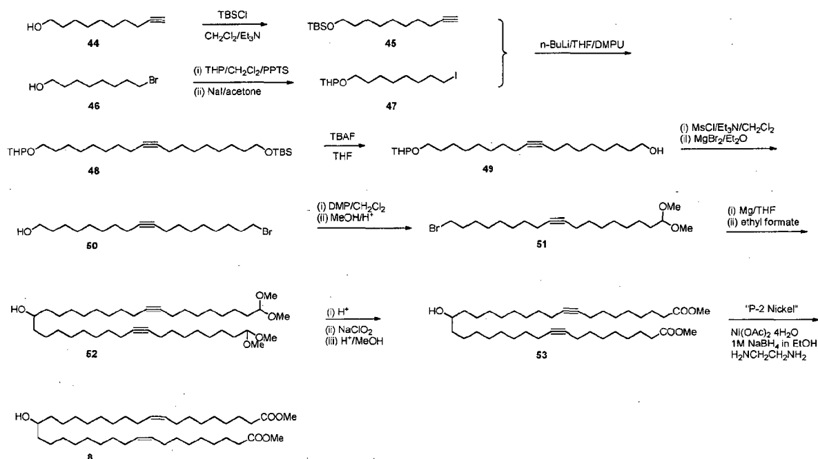
Scheme 5
