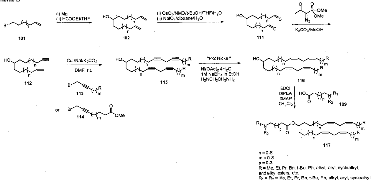
Scheme B
