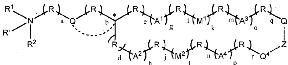
Formula (IA-2)
