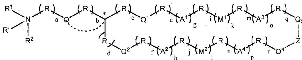
Formula (ID)
