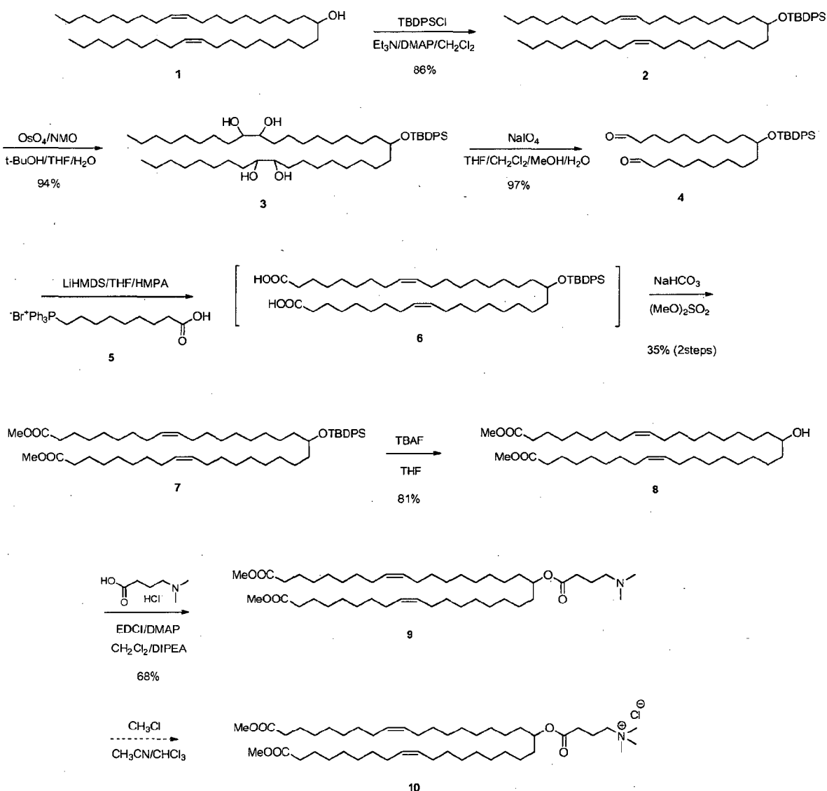
Scheme 1
