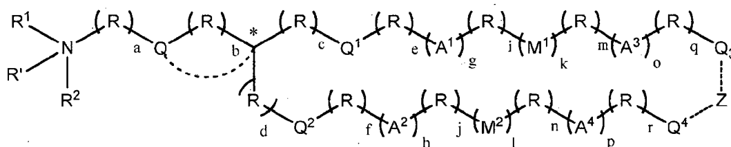
Formula (I)
