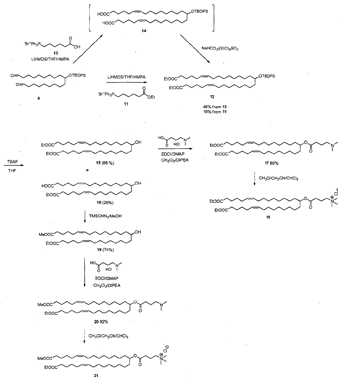
Scheme 2
