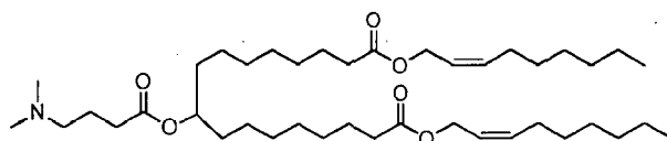
Compound 1
