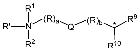
Formula (IA-1)
