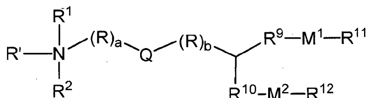
Formula (IB)
