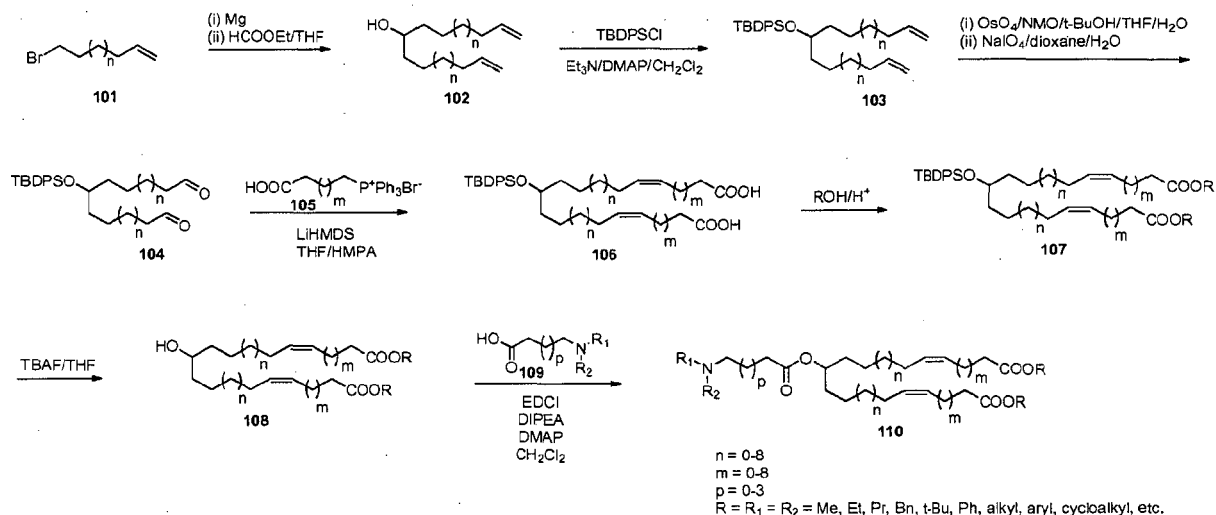
Scheme A
