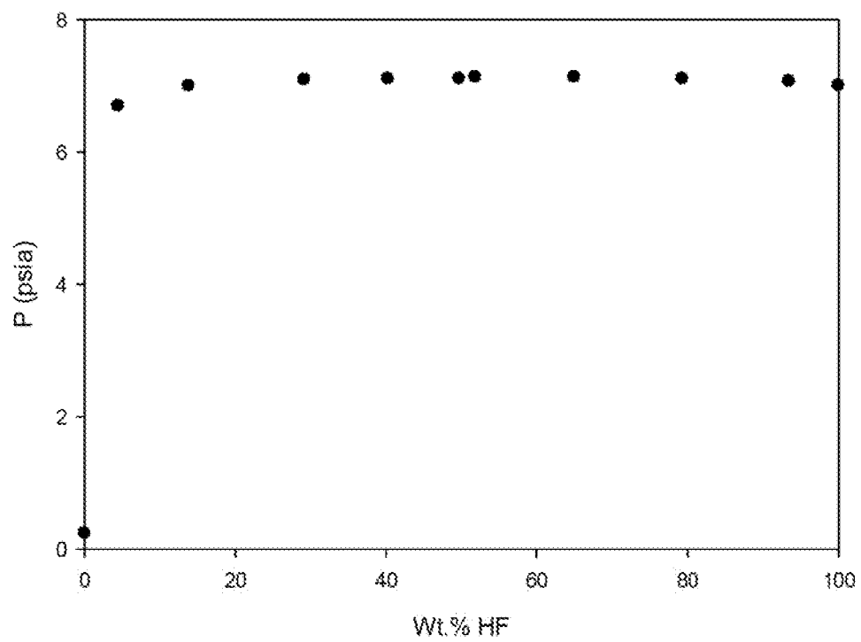
Figure 1: P-T-X of 242fa/HF at 0 C
