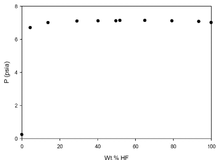
Figure 1: P-T-X of 242fa/HF at 0 C
