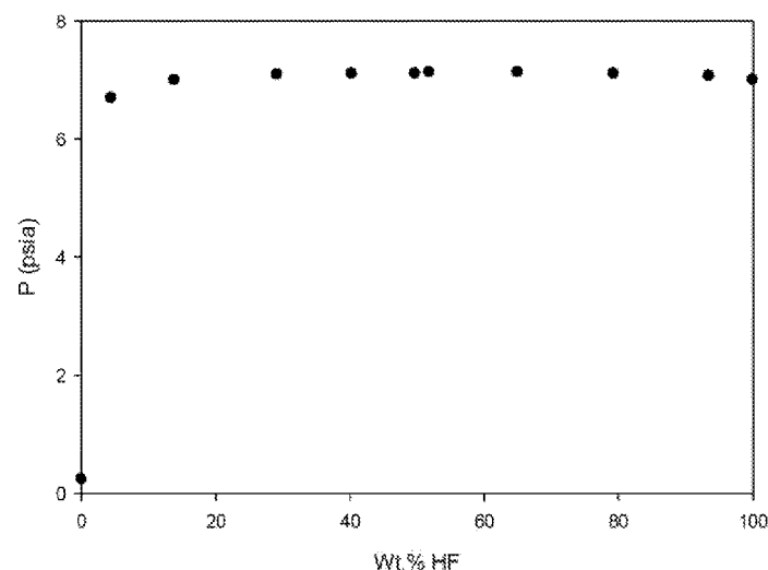
Figure 1: P-T-X of 242fa/HF at 0 C
