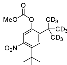
Compound 20
