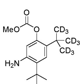
Compound 7
