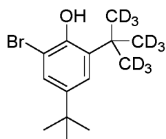
Compound 17
