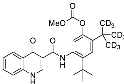
Compound 8
