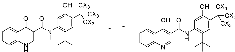
Tautomers of Formula 9
