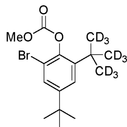
Compound 16
