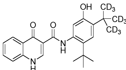
deuterated ivacaftor
