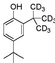
Compound 22
