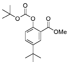
Compound 23
