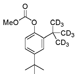
Compound 21
