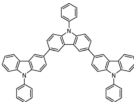
TrisPCz
