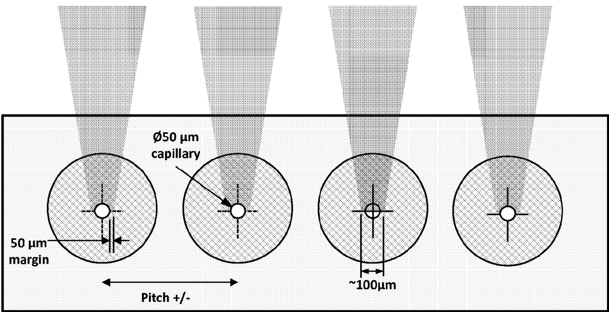
FIG. 7 Capillary cross section
