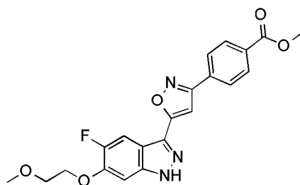
4-{5-[5-fluoro-6-(2-methoxyethoxy)-1H-indazol-3-yl]-1,2-oxazol-3-yl}benzoic acid
