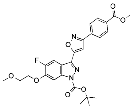
methyl 4-{5-[5-fluoro-6-(2-methoxyethoxy)-1H-indazol-3-yl]-1,2-oxazol-3-yl}benzoate
