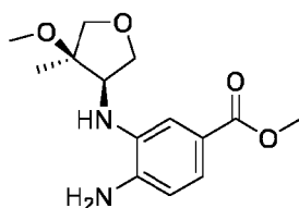
cis isomer I-1258
