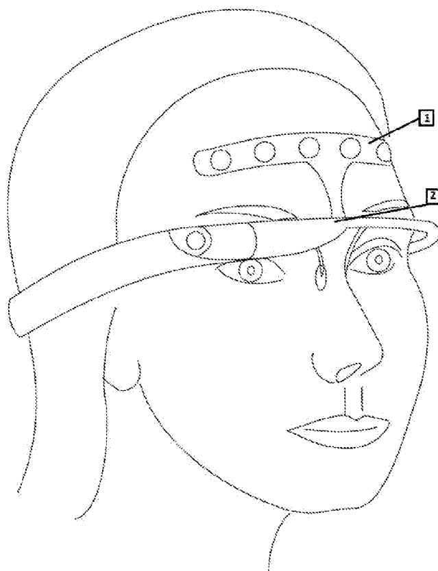
Figure 47 Simplified EEG with glasses-integrated electrode headset.
