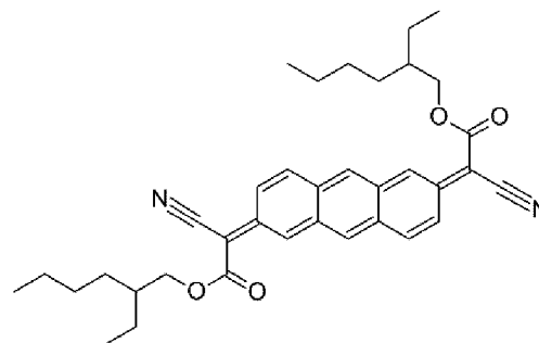
Compound 8
