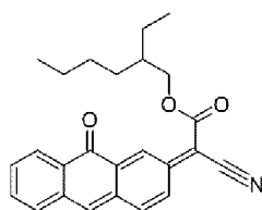
Compound 5
