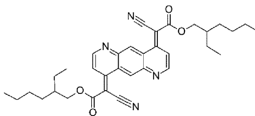
Compound 11
