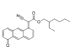
Compound 1
