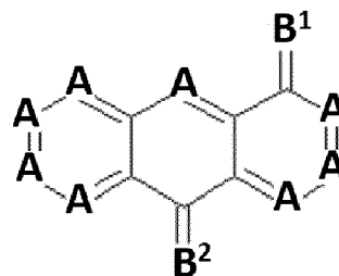
Formula IV
