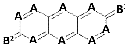
Formula II
