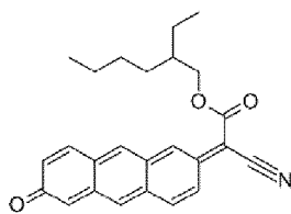
Compound 2
