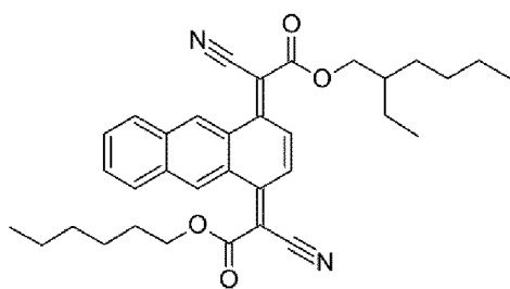
Compound 9
