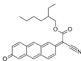
Compound 2
