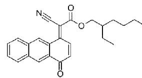
Compound 3
