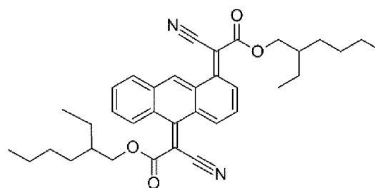
Compound 10
