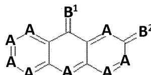
Formula V
