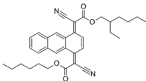
Compound 9
