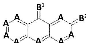
Formula V
