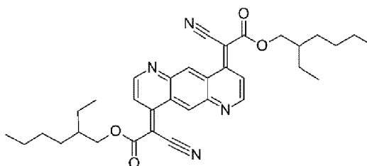
Compound 11
