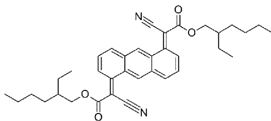
Compound 7
