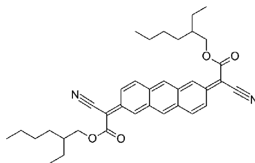
Compound 6
