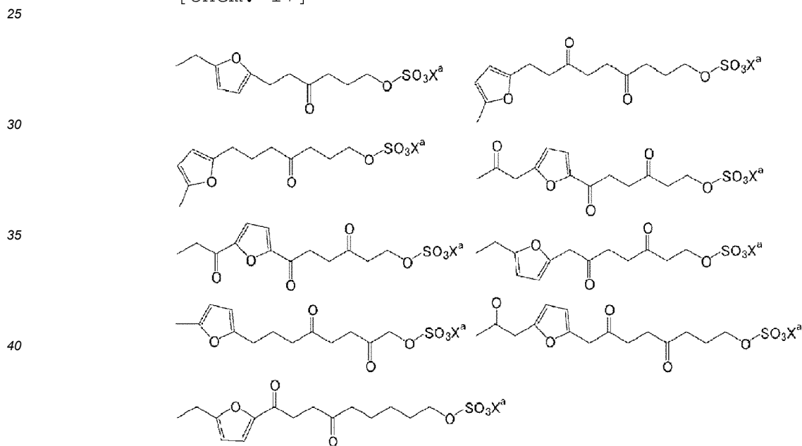
[Chem. 17]
