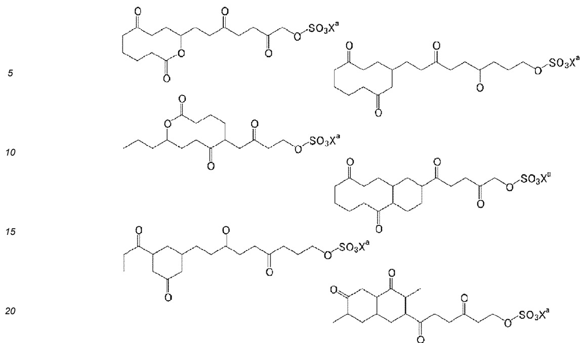
[Chem. 17]
