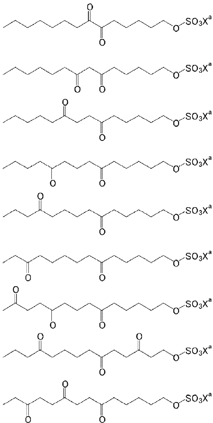
[Chem. 14]
