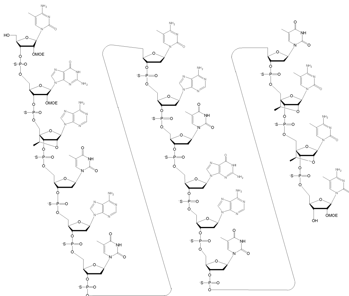
Structure 3. ISIS 548048
