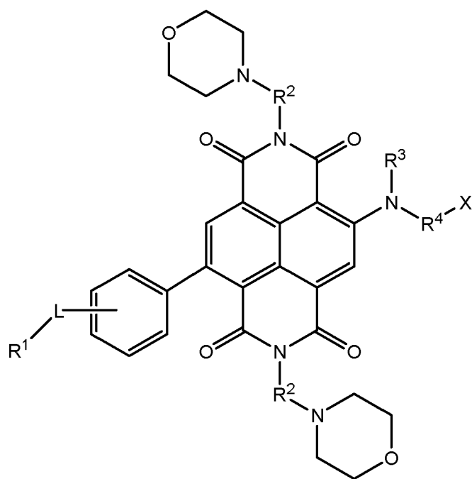
Formula I
