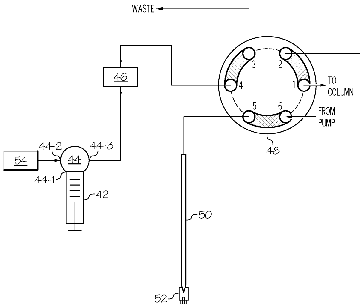
FIG. 2C (PRIOR ART)
