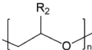
[Chemical Formula 3]
