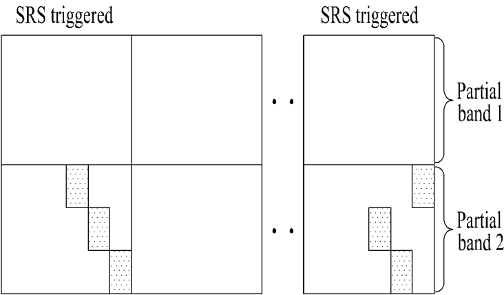
(b) another fixed symbol-level hopping pattern
