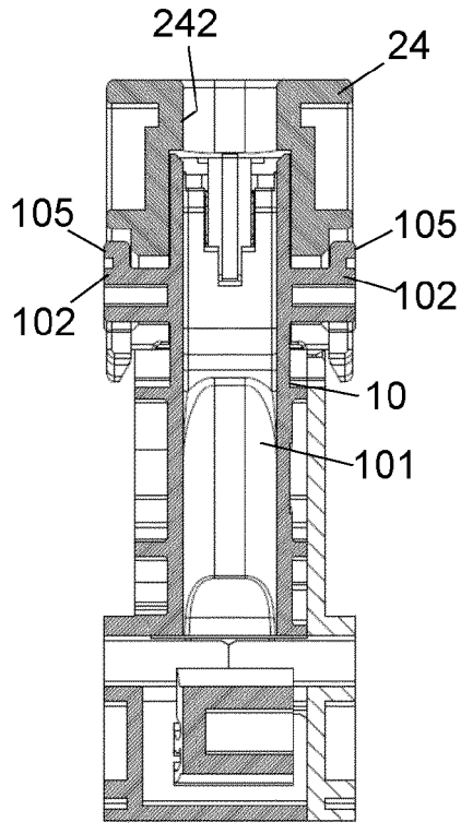
FIG 10B (B-B)
