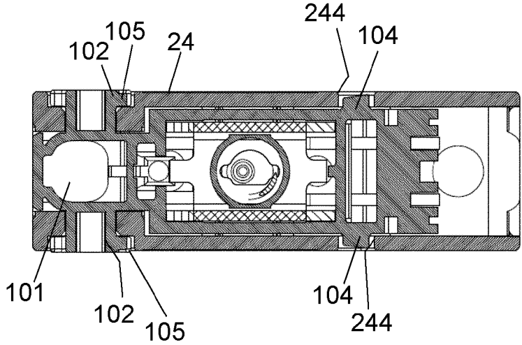
FIG 10C (C-C)
