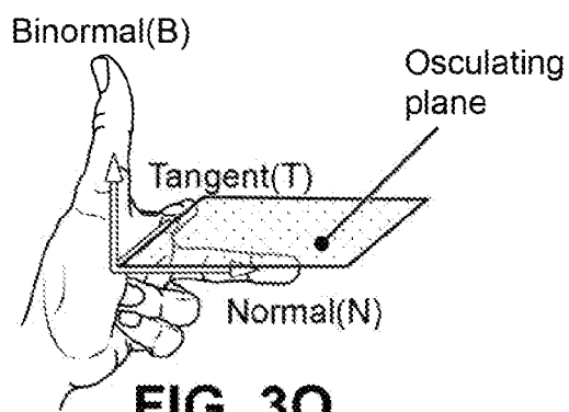
Left-hand rule
