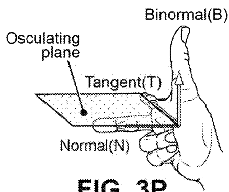
Right-hand rule
